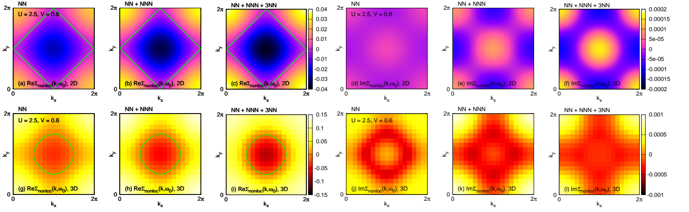
FIG. 11. (Color online) \Sigma_{\text{nonloc}}(k, i\omega_0) for the extended Hubbard model from GW + \text{EDMFT} . (a)-(f) Results for the square lattice, U = 2.5 , V = 0.80 . (g)-(l) Results for the simple cubic lattice, U = 2.5 , V = 0.60 . We only show the k_z = 0 plane. (a)-(c) and (g)-(i) \text{Re}\Sigma_{\text{nonloc}}(k, i\omega_0) . (d)-(f) and (j)-(l) \text{Im}\Sigma_{\text{nonloc}}(k, i\omega_0) . The green curves in (a)-(c) and (g)-(i) panels denote the EDMFT Fermi surface.
