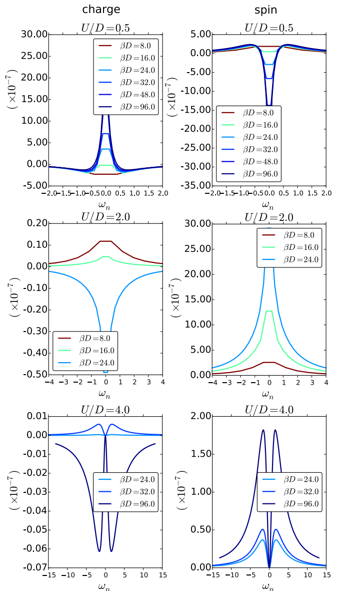
Figure 9: (color online) Evolution of \zeta^\eta(i\omega_n, i\Omega_0) on the square lattice at half filling. Left column: charge channel. Right column: spin channel. From top to bottom: U = 0.5 , U = 2.0 , U = 4.0 .
