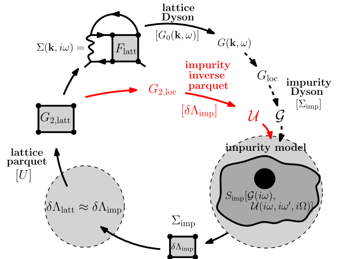
FIG. 5. The QUADRILEX loop. The parts in black correspond to the DGA in the parquet version [the dashed line shows how DGA proposes to update the Weiss field \mathcal{G}(i\omega) ]. The parts in red correspond to the additional steps necessary to update the bare impurity vertex \mathcal{U}(i\omega, i\omega', i\Omega) . For \Sigma we show only the terms beyond Hartree-Fock. The terms in square brackets denote the fixed terms in the solution of the Dyson/parquet equations.
