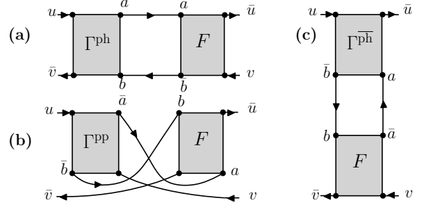
Figure 2: Graphical representation of the reducible vertex \Phi^r in the three channels. (a) \Phi^{\text{ph}} (b) \Phi^{\text{pp}} (c) \Phi^{\bar{\text{ph}}} .
