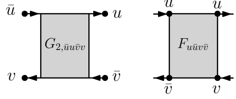
Figure 1: Graphical representation of the 4-point functions
