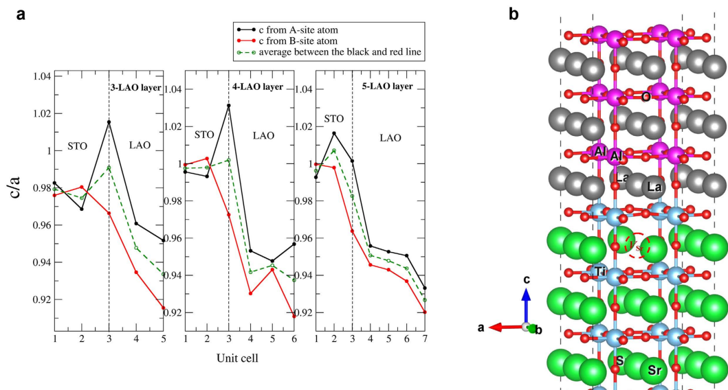
Figure 8. Modeling results. (a) Calculated c/a in non-intermixed layers of LAO on a 5 layer STO calculated in a symmetric slab geometry. (The x coordinate “3” for the black curve indicates the La-Sr distance across the interface and corresponds to the x coordinate “1” in Fig. 7). (b) Relaxation around a strontium vacancy located in the first u.c. under the interface. The V_{Sr}'' is indicated by a dashed circle. One can see the buckling of the layer above it and the O moving away from it. One can also see the La and Sr directly above the V_{Sr}'' to move toward it. The Ti-Ti distances in the c -direction surrounding the vacancy containing layer is 0.1 \text{ \AA} smaller than in the layer below it without vacancy.
