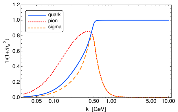
Figure 10: Dimensionless RG-invariant propagators as functions of the RG scale.
