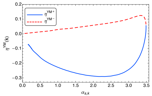
Figure 3: The UV and IR branches of \eta_{A,k}^{\text{YM}}(k) , which is defined in (51).
