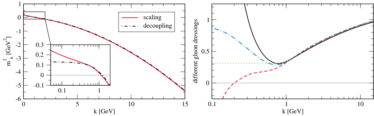
FIG. 10. Left: Gluon mass parameter m_k^2 = \Gamma_{AA,k}^{(2)}(p=0) over k . Right: Possible choices for the scaling prefactor in the gluon regulator: Z_{A,k}(k) (black, solid), \bar{Z}_{A,k}(k) (red, dashed), \hat{Z}_{A,k}(k) (blue, dot-dashed) and \tilde{Z}_{A,k} (green, dotted) as defined in (E3) and (E5). Independence of the results from the above choice has been checked explicitly.
