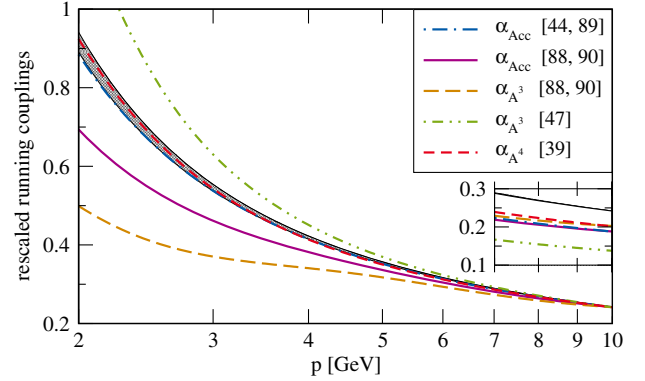
FIG. 7. Running couplings (20) in comparison with DSE running. The grey band gives the spread of vertex couplings from the FRG in the present work. The DSE results are shown rescaled to fit our ghost-gluon vertex running coupling at 10 GeV to facilitate the comparison. The inlay shows the unscaled couplings. Note that the FRG running couplings naturally lie on top of each other and are not depicted rescaled.
