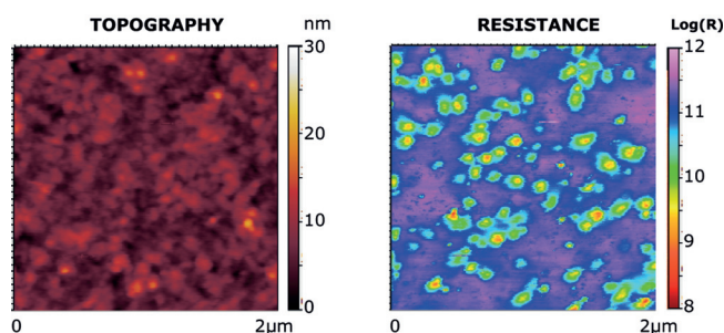
FIG. 5. Typical topography and resistance maps obtained by PFM-Resiscope with a PtIr-coated tip ( -3 \text{ V} biased) on a P3HT:PCBM solar cell active layer on ITO/glass substrate.
