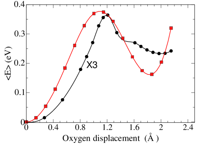
FIG. 3: Calculated average total Energy per atom in eV as a function of oxygen displacement in ( \text{\AA} ) with total atomic relaxation (black dots) compared to the unrelaxed structure (red dots). Notice that the atomic relaxation reduces drastically the energy barrier height.
