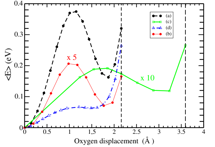
FIG. 2: Average total Energy per atom in eV as a function of oxygen displacement in ( \text{\AA} ) for the several cases of oxygen motion : (a) small unit cell; (b) large unit cell and only one oxygen is allowed to move; (c) large unit cell, V vacancy; (d) small unit cell, V on top of Mg. Cases (b) and (c) are amplified 5 and 10 times respectively. All the cases are performed within the LDA approximation. The origin of the displacement corresponds to the position of the last MgO layer, the dashed line at 2.16 \text{\AA} refers to the first vanadium layer and the dashed line at 3.593 \text{\AA} to the second one.
