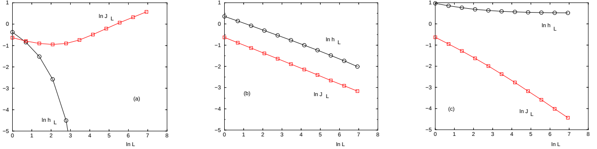
FIG. 1: RG flows in log-log scale of the typical renormalized transverse field h_L^{typ} (circles) and of the renormalized coupling J_L^{typ} (squares) for \sigma = 0.625 :
