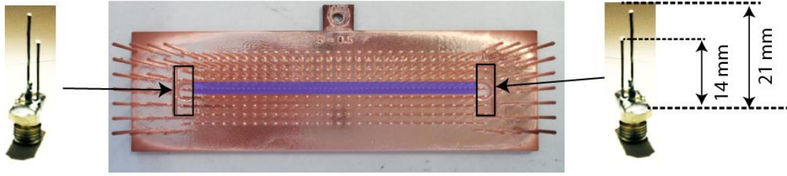
Figure S4| Picture of a device and of the home-made antennas. The waveguide defect wires are highlighted in blue and the holes for antennas in solid black rectangles. Photographs of the home made antennas used for spectral and temporal measurements with the feed antenna of 21 mm and the extra defect wire of 14 mm (sides).
