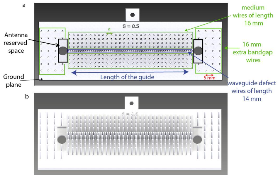
Figure S2| CAD views of a typical device. a, top, b, perspective
