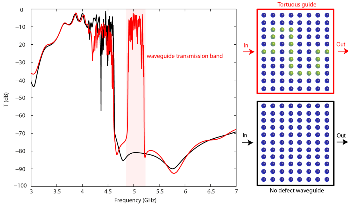
Figure S3| Simulated transmission through the tortuous waveguide of Figure 1. Simulated transmission through the waveguide (red) and through the medium with no defect line waveguide (black) along with schematics of the two simulated devices (blue dots = wires of the medium, green dots = defect wires).
