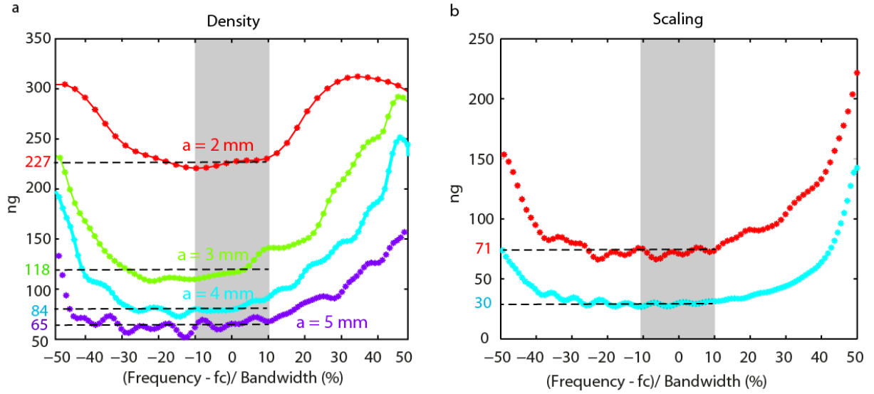
Figure S6| Experimental broadband measurements of the group index. a , samples of Figure 3a and b , samples of Figure 4b. Data are plotted as a function of the frequency, centered on f_c and normalized by the bandwidth. The x-axis is presented as a percentage of the bandwidth. The frequency range on which the group index displayed in the main text is averaged is shaded in grey, while the corresponding value is advised on the y-axis.
