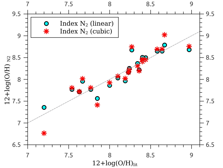
Fig. 1. Oxygen abundances calculated from raw spectral data by using both fits to the \text{N}_2 ratio given by Pettini & Pagel (2004), as a function of the abundances taken directly from the literature. Cyan dots (red stars) correspond to the linear (cubic) calibration of the \text{N}_2 index; the dashed line represents the identity.
