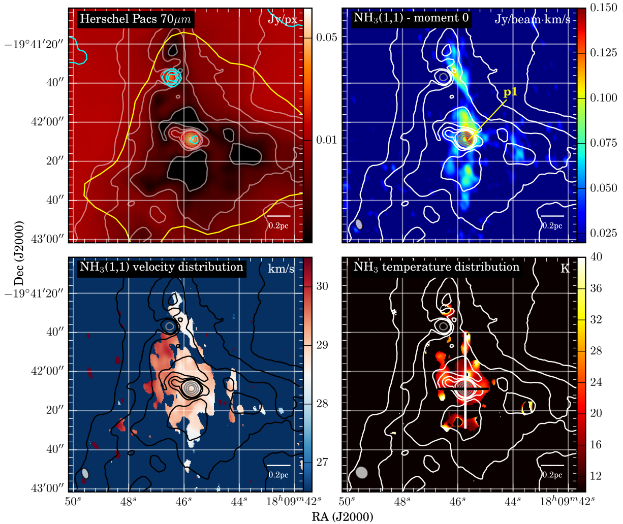
Fig. 1. IRDC010.70 – overview. Upper left panel: Herschel PACS 70 \mu\text{m} emission and cyan contours present Spitzer MIPS 24 \mu\text{m} emission at levels of 90, 110, 130, and 150 MJy/sr. The yellow contour shows the 3-sigma limit of the SCUBA 850 \mu\text{m} emission and therefore the area where we measured the clump mass. Following panels: VLA data. Upper right panel: integrated emission of the main \text{NH}_3(1,1) line in \text{Jy beam}^{-1} \text{km s}^{-1} from 27.1 to 30.3 \text{km s}^{-1} . Lower left panel: peak velocity distribution in \text{km s}^{-1} . Lower right panel: kinetic temperature in K. We extracted the temperature distribution along the black and white lines shown in the lower right panel and plotted the values as a function of distance in Fig. 10. In each panel contours present Herschel PACS 70 \mu\text{m} emission at levels of 2.5, 5, 7.5, and 10 mJy/px for white/black contours and 20, 30, 40, and 50 mJy/px for gray contours. The \text{NH}_3(1,1) emission peak is marked in the upper right panel, and the corresponding spectra are given in Fig. A.1. The synthesized beam and scale are shown in each panel.
