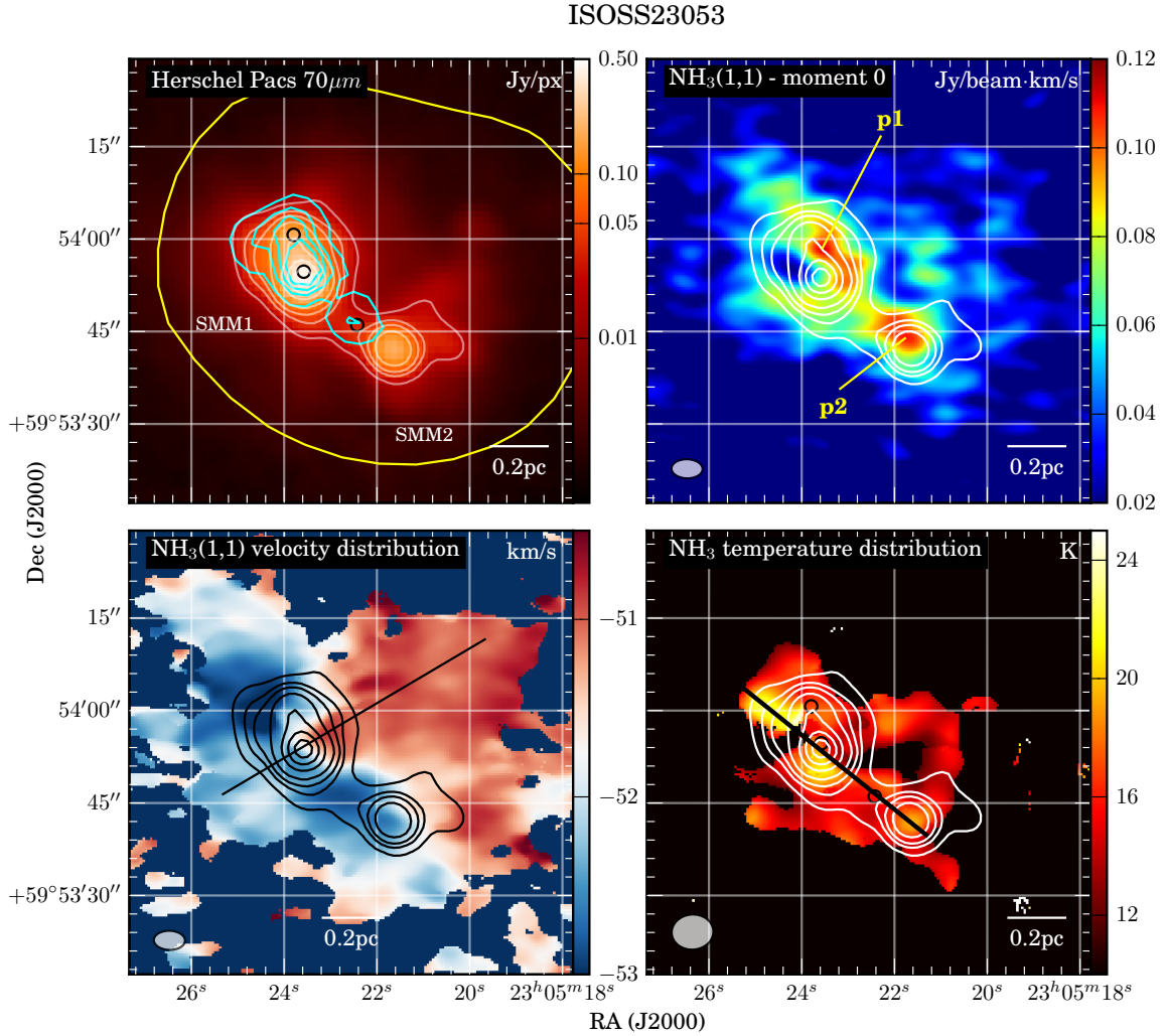
Fig. 6. ISOSS23053 – overview. Upper left panel: Herschel PACS 70 \mu\text{m} emission, and cyan contours present Spitzer MIPS 24 \mu\text{m} emission at levels of 75, 150, 225, and 300 MJy/sr. The yellow contour shows the 3-sigma limit of the SCUBA 850 \mu\text{m} emission and therefore the area where we measured the clump mass. Following panels: VLA and Effelsberg 100 m Telescope data combined. Upper right panel: integrated emission of the main \text{NH}_3(1,1) line in \text{Jy beam}^{-1} \text{km s}^{-1} from -53.3 to -50.1 \text{ km s}^{-1} . Lower left panel: peak velocity distribution in \text{km s}^{-1} , and the black line indicates the direction of the position-velocity cut shown in Fig. 7. Lower right panel: kinetic temperature in K. We extracted the temperature distribution along the black line shown in the lower right panel and plotted the values as a function of distance in Fig. 10. The black circles indicate Spitzer MIPS 24 \mu\text{m} emission sources. In each panel white/black contours present Herschel PACS 70 \mu\text{m} emission at levels of 20, 40, 60, 100, 200, 300, and 400 mJy/pixel. The \text{NH}_3(1,1) emission peaks are marked in the upper right panel, and the corresponding spectra are given in Fig. A.6. The synthesized beam and scale are shown in each panel.
