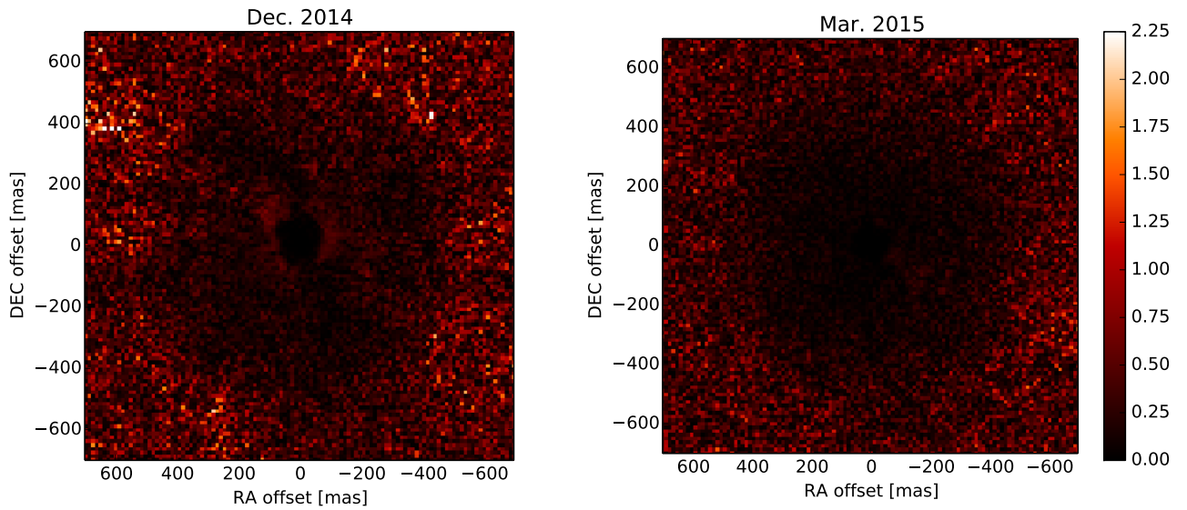
Fig. A.1. U_\phi images (left, December 2014; right, March 2015). East is toward the left. Each pixel has been scaled with the square of its distance from the star, r^2 , to compensate for the r^{-2} dependency of the stellar illumination. The color scale is arbitrary.
