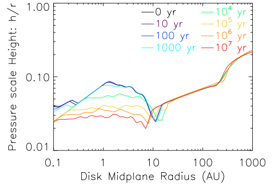
Fig. 6. Evolution of the pressure scale height as a function of the radial distance for an initial minimum mass solar nebula in the case of a self-consistently calculated geometry with a full continuous model of opacities.
