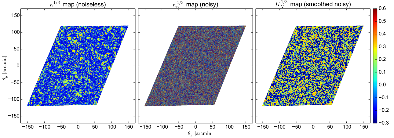
Fig. 3. Patch of a map projected with regard to its center, taken from a realization of fast simulations. The left, middle, and right panels give the fields \kappa^{1/3} , \kappa_n^{1/3} , and K_N^{1/3} , respectively. We have taken the cubic root to emphasize the contrast. It is clear that the signal is completely dominated by the noise. Even though the smoothed map is quite different from the original one, the structures, high-signal regions are still conserved and traced.
