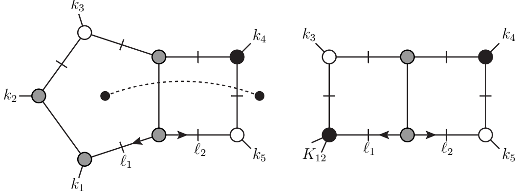
Figure 19. The one-mass bow-tie hexacut embeds several genuine two-loop integrals. Our basis includes the dual conformal pentabox and the one-mass double box. The figure shows a particular kinematical configuration.
