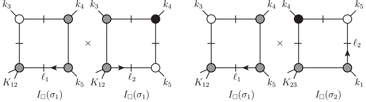
Figure 18. Products of one-loop one-mass box integrals which cannot support a pentabox octacut (since the propagator (\ell_1 - k_1) is absent), but may contribute to double-box octacuts, i.e. residues from Jacobian poles. The figure shows a particular configuration of chiral, antichiral and nonchiral vertices.
