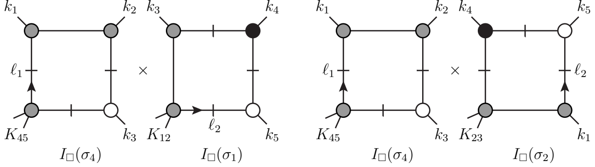
Figure 17. Products of one-loop one-mass box integrals which can support a pentabox octacut. A one-mass box with a massive corner K_{12} is identified with the standard ordering (12345), in agreement with the conventions for the two-loop integrals. The figure shows a particular branch of the hexacut.
