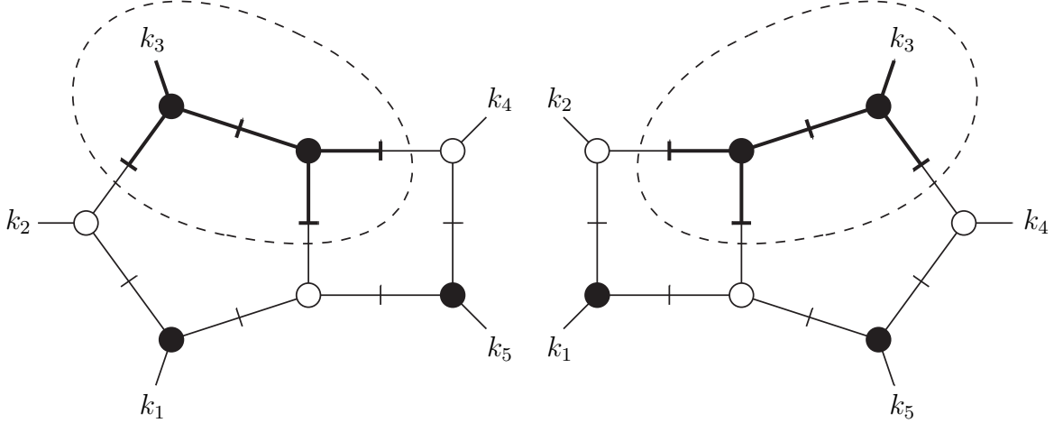
Figure 12. The octacut global poles \mathcal{G}_3 (left) and \mathcal{G}_2 (right) of respectively P_{3,2}^{**}(\sigma_1) and P_{3,2}^{**}(\sigma_3) . The encircled subdiagrams are related by the split-and-merge operation.
