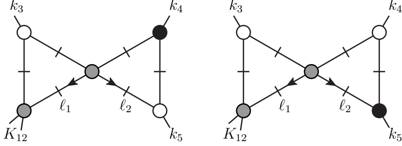
Figure 16. The one-mass bow-tie hexacut, which has two pairs of parity conjugate branches. This figure only shows branches that are not related to each other by parity conjugation. All internal lines are on-shell.
