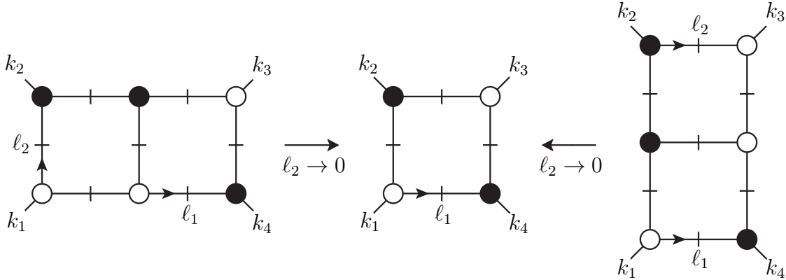
Figure 4. A second example of how a global pole could be shared between the horizontal and vertical double-box integrals.
