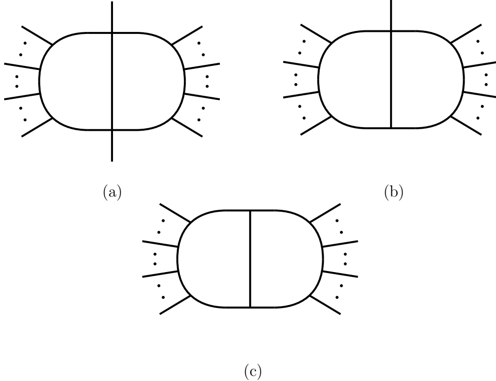
Figure 1. The three basic types of two-loop planar integrals, labeled by the number of legs attached to each internal line of the vacuum diagram: (a) P_{n_1, n_2} , (b) P_{n_1, n_2}^* , (c) P_{n_1, n_2}^{**} .
