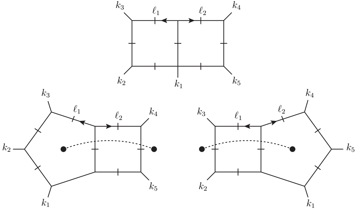
Figure 14. There is a second turtle-box heptacut which also receives contributions from two cyclic permutations of the pentabox. The dashed lines in the left and right diagrams indicate numerator insertions of (\ell_1 + k_4)^2 and (\ell_2 + k_3)^2 respectively.
