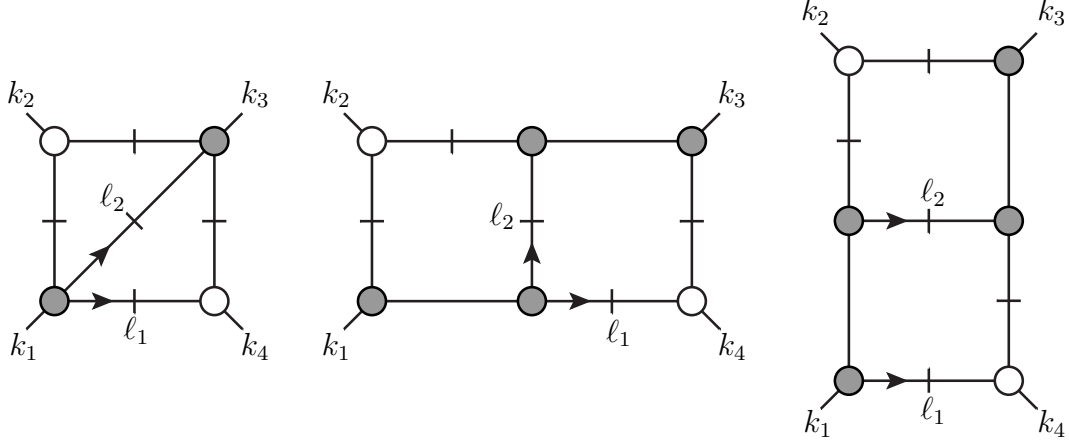
Figure 7. The pentacut provides a natural prescription for aligning the loop-momentum labels in different integrals. The global octacut poles of the double-box integrals can be analyzed by performing a further three-dimensional contour integral on the pentacut slashed-box integral at left. The gray blobs indicate vertices of indefinite chirality.
