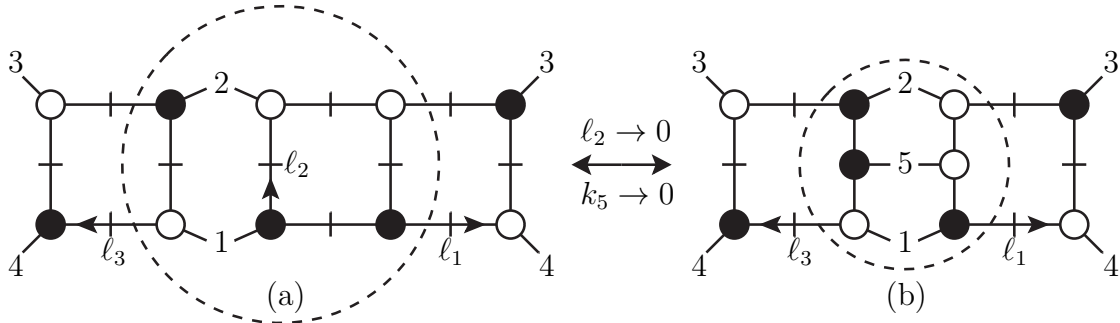
Figure 6. Two maximal unitarity cuts for diagrams that enter the cross section at the same order in the coupling: (a) a one-loop times two-loop contribution and (b) a one-loop squared contribution. These cuts share the same kinematical configuration in the indicated soft limits. The encircled subdiagrams correspond precisely to the sharing of poles illustrated in fig. 5.
