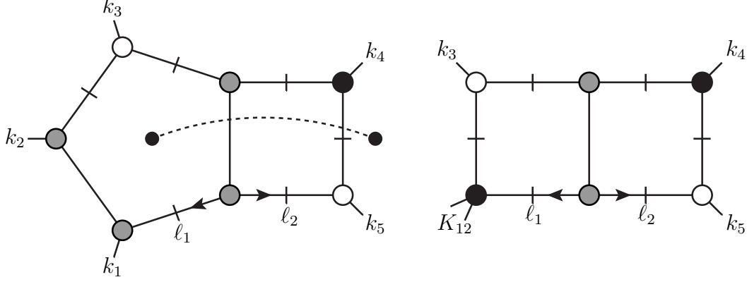
Figure 19. The one-mass bow-tie hexacut embeds several genuine two-loop integrals. Our basis includes the dual conformal pentabox and the one-mass double box. The figure shows a particular kinematical configuration.
