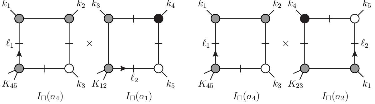
Figure 17. Products of one-loop one-mass box integrals which can support a pentabox octacut. A one-mass box with a massive corner K_{12} is identified with the standard ordering (12345), in agreement with the conventions for the two-loop integrals. The figure shows a particular branch of the hexacut.
