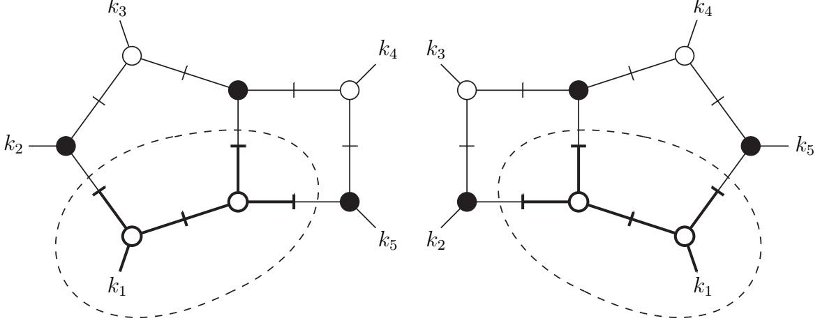
Figure 15. The octacut global poles \mathcal{G}_1 and \mathcal{G}_2 in P_{3,2}^{**}(\sigma_1) are shared with P_{3,2}^{**}(\sigma_4) . As the poles are related by parity conjugation, only diagrams relevant for \mathcal{G}_1 are shown. The four-point subdiagram which is responsible for the sharing is marked by thicker lines and surrounded by a dashed circle.
