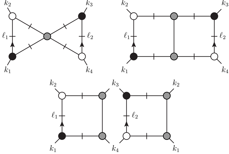
Figure 8. The bow-tie hexacut detects contributions from both the planar double box and squared one-loop boxes. This figure shows a particular example where vertices at opposite corners have equal chiralities in the bow-tie diagram.
