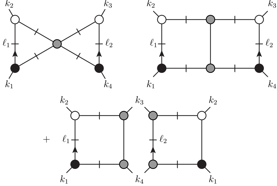
Figure 9. The second inequivalent type of bow-tie hexacut considered in the main text, with contributions from the double box and a squared box.
