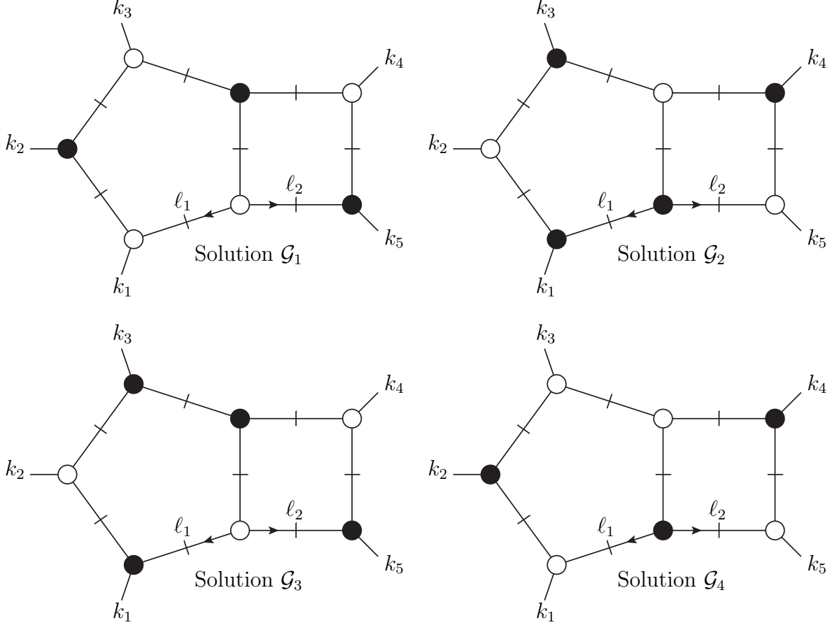
Figure 10. The four octacut solutions for the massless pentabox. In our notation, as in prior figures, chiral and antichiral vertices are depicted by white and black blobs respectively, following for example the conventions of ref. [79]. Each of these four solutions is associated with a unique point in \mathbb{CP}^4 \times \mathbb{CP}^4 .
