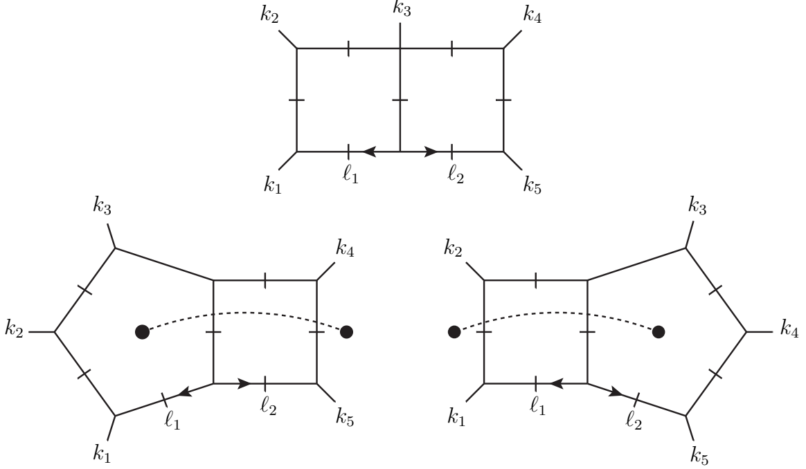
Figure 13. The two displayed permutations of the pentabox share a turtle-box heptacut. This is evident directly from the diagrams because the four-point vertex of the turtle box can be opened to a pair of three-point vertices to either loop.
