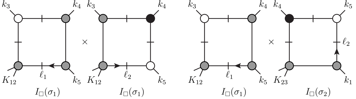
Figure 18. Products of one-loop one-mass box integrals which cannot support a pentabox octacut (since the propagator (\ell_1 - k_1) is absent), but may contribute to double-box octacuts, i.e. residues from Jacobian poles. The figure shows a particular configuration of chiral, antichiral and nonchiral vertices.
