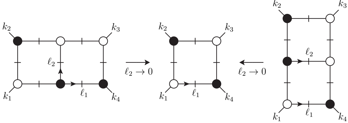
Figure 2. An example of a global pole shared between the horizontal and vertical double-box integrals. The loop momentum labeling is chosen cunningly. At the global pole, the nonvanishing heptacut propagator momentum in each double box corresponds to that of a quadruply cut one-loop box. The white and black blobs indicate chiral (MHV) and antichiral ( \overline{\text{MHV}} ) vertices, respectively, as in the conventions (for example) of ref. [79].
