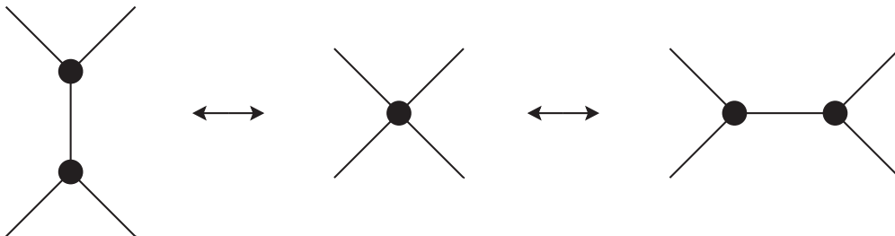
Figure 11. The merge-and-split operation applied to two adjacent antichiral vertices.
