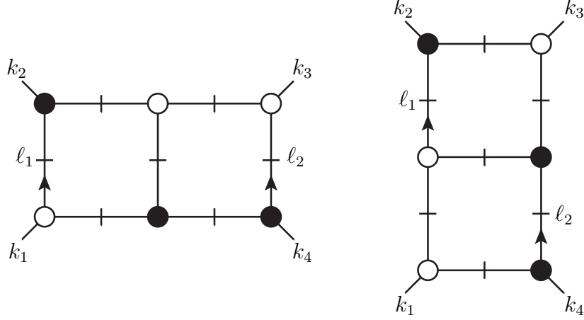
Figure 3. The horizontal and vertical double boxes. All internal lines are on-shell.
