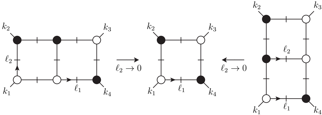
Figure 5. A third example of how a global pole could be shared between the horizontal and vertical double-box integrals.
