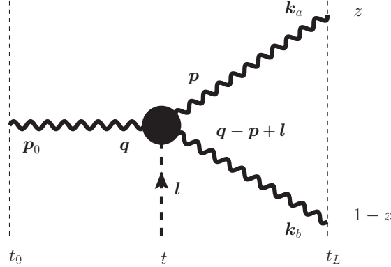
Figure 3. Graphical illustration of the equation (4.2). The thick wavy lines represent the probability \mathcal{P} for transverse momentum broadening, the black dot is the splitting kernel \mathcal{K} .
