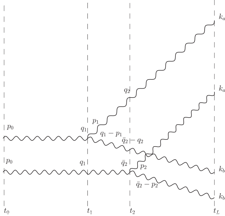
Figure 4. The momenta of the intermediate states in Eq. (A.3). The amplitude is drawn above the complex conjugate amplitude (see Ref. [20]), with the gluon splitting occurring at time t_1 in the amplitude, and at time t_2 in the complex conjugate amplitude. At any given time, the sum of momenta in the amplitude equals that of momenta in the complex conjugate amplitude.
