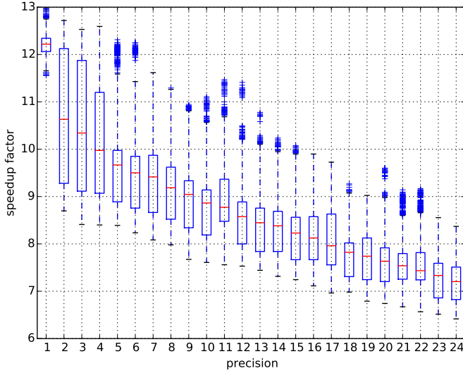
(a) Speedup
