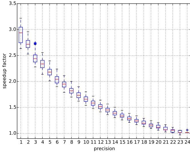
(a) Speedup
