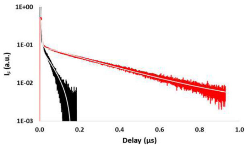
Figure 4. Fluorescence decays of (R)-1 in aerated (black) and argon-purged toluene solutions (red); the solid (white) lines are the biexponential fits ( \lambda_{\text{ex}} = 400 \text{ nm} ).
