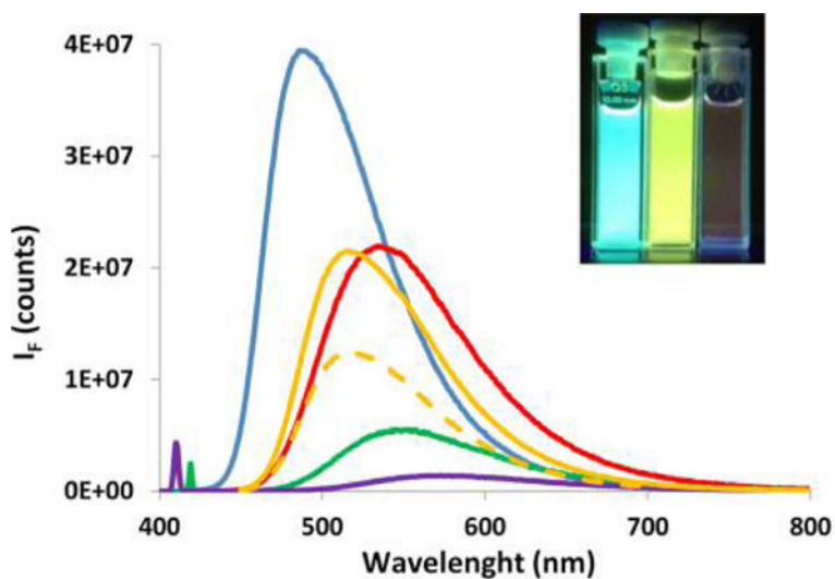
Figure 3. Fluorescence spectra ( C = 10^{-5} M) of ( R )- 1 in cyclohexane (blue), THF (red), nondegassed toluene (orange dashed line) and argon degassed (orange solid line), dichloromethane (green), and ethanol (purple); \lambda_{ex} = 410 nm. Inset picture: fluorescence under 365 nm excitation of ( R )- 1 in cyclohexane, THF, and ethanol (from left to right).
