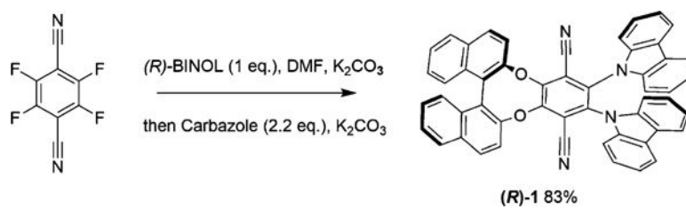
Scheme 1. One-Pot Sequential Synthesis of ( R )-1
