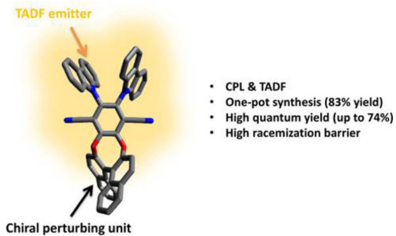
Figure 1. Molecular design of 1 .
