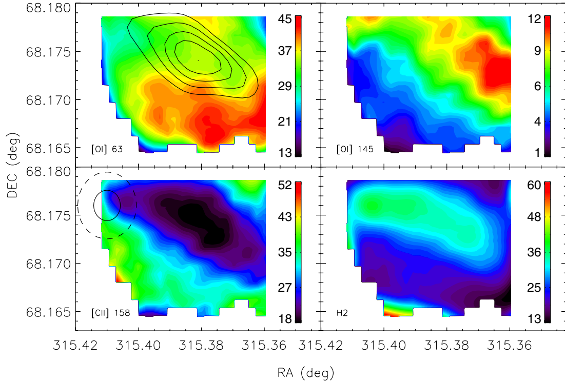
Fig. 6. Relative cooling budget of the [O I]63 and 145 \mu\text{m} , [C II]158 \mu\text{m} lines, and the 0-0 S(1), S(2), S(3) H 2 rotational transitions and v = 1-0 S(1) in percentage (%). Adding the contribution of all four species for a given point in the map amounts to 100%. Other species that can contribute to the cooling are ignored in this figure (see Sect. 4). In the first panel we show a contour of the PDR as traced by the [O I]63 \mu\text{m} emission to guide the eye. The images have been convolved to the largest of the beam sizes of these species, in this case the [C II]158 \mu\text{m} line, shown as a solid circle in the [C II] panel. In addition, and for comparison, we also show the largest CO beam size (25'') used to calculate the cooling budget in Table 1 as a dashed circle.
