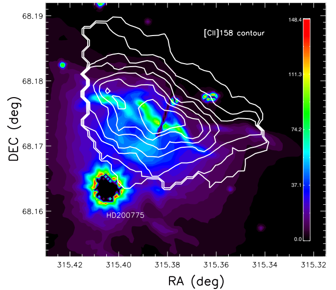
Fig. 4. Comparison of the PAH morphology as traced by the IRAC 3.6 μm band intensity in MJy/sr (taken from the Spitzer archive), with [C II] 158 μm in white contours. In decreasing order the contour levels are at 10.1, 9.0, 7.8, 6.7, 5.6, 4.5, 3.4, and 2.2 \times 10^{-7} \text{ W m}^{-2} \text{ sr}^{-1} .
