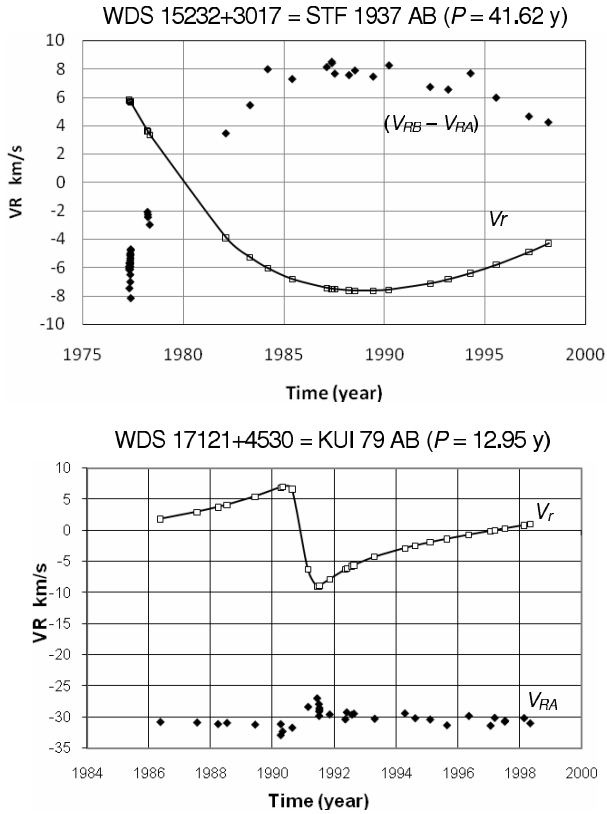
Fig. B.2. Examples of lifting the ambiguity on the ascending node for a visual binary. Top (cases 2, 5 of Table B.1): the slope of the computed \tilde{V}_r curve is opposite to that of the V_r(\text{B})-V_r(\text{A}) measurements: it is then necessary to add 180^\circ to the values of \Omega and \omega given by the 6th Catalog of Orbits of Visual Binary Stars (6th COVBS; Hartkopf et al. 2001). Bottom (cases 3, 6 of Table B.1): the slope of the computed \tilde{V}_r curve is opposite to that of V_r(\text{A}) measurements; there is no need to change the values of \Omega and \omega listed in the 6th COVBS.
