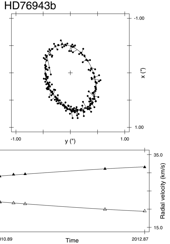
Fig. A.4. Combined astrometric ( upper panel ) and spectroscopic ( lower panel ) orbits for WDS 09006+4147AB. Filled triangles in the lower panel refer to component A. Individual measurements for the visual orbit were taken from the WDS database.
