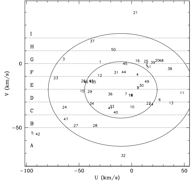
Fig. 9. Distribution of the systems in the (U, V) plane, with the same labels as in Fig. 1. System 17 (01083+5455) falls outside the boundaries, at U = -43 km s ^{-1} and V = -157 km s ^{-1} . To fix the ideas, two velocity ellipsoids are shown, both centred on the reflex solar motion in the LSR: -U_\odot = -10.2 km s ^{-1} , -V_\odot = -20.5 km s ^{-1} , and with \sigma_U = 34.5 km s ^{-1} , \sigma_V = 22.5 km s ^{-1} , as derived by Famaey et al. (2005) from their most precise sample. Horizontal bands and the corresponding labels are used in Fig. 10.
