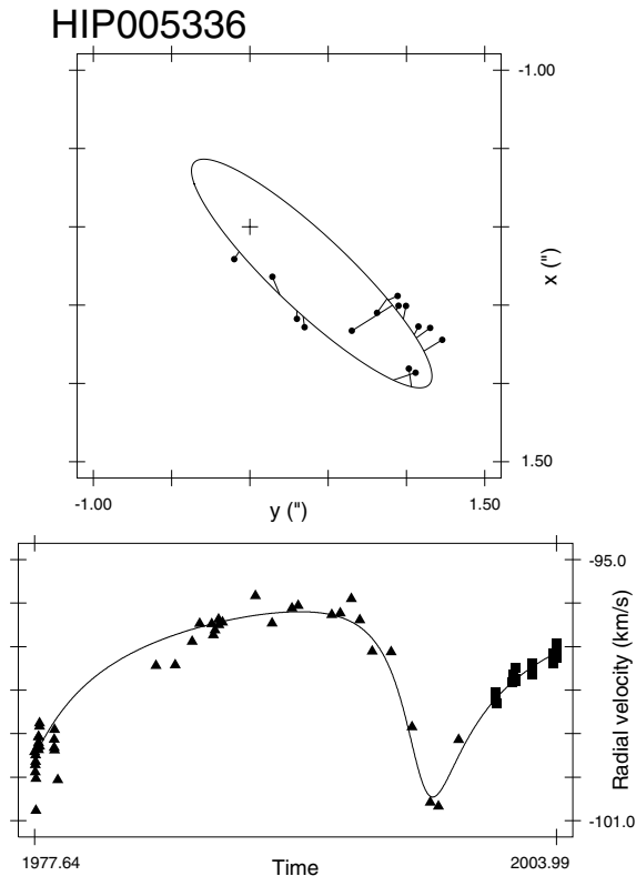
Fig. A.2. Combined astrometric ( upper panel ) and spectroscopic ( lower panel ) orbits for WDS 01083+5455Aa,Ab = HIP 5336 = HD 6582 = \mu Cas. The solid line in the lower panel corresponds to the predicted velocity curve for A. Triangles are CORAVEL measurements, squares are measurements from Abt & Willmarth (2006) . Individual measurements for the visual orbit were taken from the WDS database.
