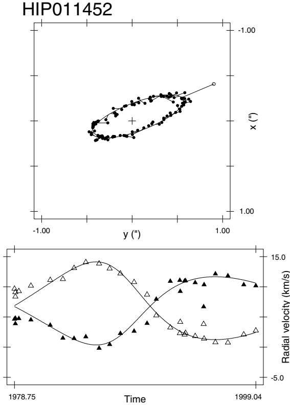
Fig. A.3. Combined astrometric ( upper panel ) and spectroscopic ( lower panel ) orbits for WDS 02278+0426AB. In the lower panel , filled and open triangles correspond to CORAVEL velocities for components 1 and 2, respectively. Individual measurements for the visual orbit were taken from the WDS database at USNO.
