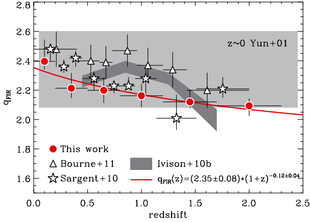
Fig. 9. Evolution of the L_{\text{FIR}} to -L_{1.4\text{GHz}} ratio, q_{\text{FIR}} , with redshift, as inferred from our stacking analysis. Red circles and error bars correspond to the median and interquartile range observed in our study in regions of the parameter space not affected by incompleteness (green dashed lines in Fig. 8). The red line corresponds to a redshift-dependent fit to our data points, q_{\text{FIR}}(z) = 2.35 \times (1+z)^{-0.12} . The light grey region shows the value of q_{\text{FIR}} observed by Yun et al. (2001) in a large sample of local star-forming galaxies, q_{\text{FIR}}(z \sim 0) = 2.34 \pm 0.26 . This local measurement is displayed over the entire range of redshift to highlight any possible redshift evolution of q_{\text{FIR}} . The dark grey region presents results from Iverson et al. (2010b) using Herschel observations on a L_{\text{IR}} -matched sample. Empty triangles show results from Bourne et al. (2011), as inferred using a stacking analysis on a stellar-mass-selected sample of galaxies. Stars present results obtained by Sargent et al. (2010) using a FIR/radio-selected sample of star-forming galaxies and applying a survival analysis to properly treat flux limits from non-detections.
