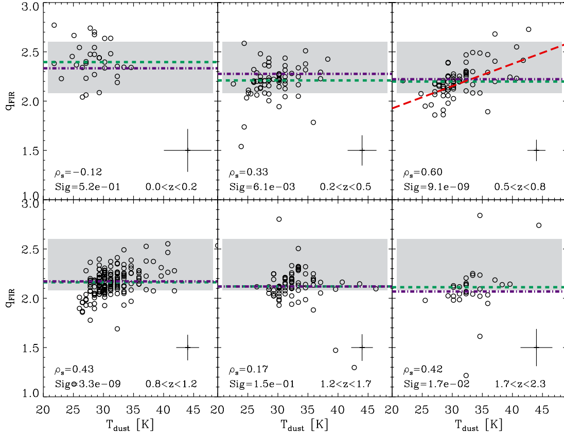
Fig. 10. Mean L_{\text{FIR}} – to – L_{1.4\text{GHz}} ratio ( q_{\text{FIR}} ) of galaxies as a function of dust temperature, as derived from our stacking analysis. In each panel, we give the Spearman rank correlation ( \rho_s ), the null hypothesis probability (Sig.), and show the median uncertainties on our q_{\text{FIR}} and T_{\text{dust}} estimates. In the redshift bin with a statistically significant (Sig. < 5% and \chi^2_{\text{red}}[\text{linear}] < \chi^2_{\text{red}}[\text{cst}] ) correlation, we plot (red long-dashed lines) a linear fit, q_{\text{FIR}} = (0.023 \pm 0.008) \times T_{\text{dust}} + (1.47 \pm 0.32) . The rest of the lines and shaded region are the same as in Fig. 8.
