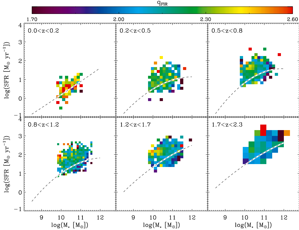
Fig. 7. Evolution of the mean L_{\text{FIR}} - \text{to} - L_{1.4\text{GHz}} ratio, i.e. q_{\text{FIR}} (see Eq. (5)), of galaxies in the SFR– M_* plane, as found using our stacking analysis. Short-dashed lines on a white background show the MS of star formation.
