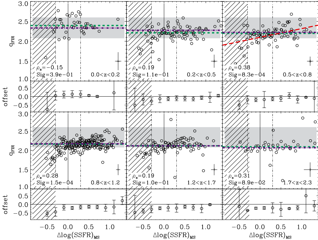
Fig. 8. Mean L_{\text{FIR}} – to -L_{1.4\text{GHz}} ratio ( q_{\text{FIR}} ) of galaxies as a function of \Delta\log(\text{SSFR})_{\text{MS}} , as derived from our stacking analysis. Hatched areas represent the regions of parameter space affected by incompleteness (see text and Fig. 4), while the light grey region shows the value of q_{\text{FIR}} observed by Yun et al. (2001) in a large sample of local star-forming galaxies, q_{\text{FIR}}(z \sim 0) = 2.34 \pm 0.26 . In each panel, we show the median value (green dashed line), give the Spearman rank correlation ( \rho_s ) and the null hypothesis probability (Sig.) derived from data points in the region of parameter space not affected by incompleteness. Blue dot-dashed lines represent a redshift evolution of q_{\text{FIR}} = 2.35 \times (1+z)^{-0.12} . In the lower right part of each panel, we give the median uncertainty on our q_{\text{FIR}} estimates. Vertical solid and dot-dashed lines show the localisation and the width of the MS of star formation. In the redshift bin with a statistically significant correlation (Sig. < 5% and \chi^2_{\text{red}}[\text{linear}] < \chi^2_{\text{red}}[\text{cst}] , see text), we plot (red long-dashed line) a linear fit, q_{\text{FIR}} = (0.22 \pm 0.07) \times \Delta\log(\text{SSFR})_{\text{MS}} + (2.10 \pm 0.05) . The lower panel of each redshift bin shows the offset between the median q_{\text{FIR}} of our data and the local value of q_{\text{FIR}}(z = 0) \approx 2.34 , in bins of 0.2 dex.
