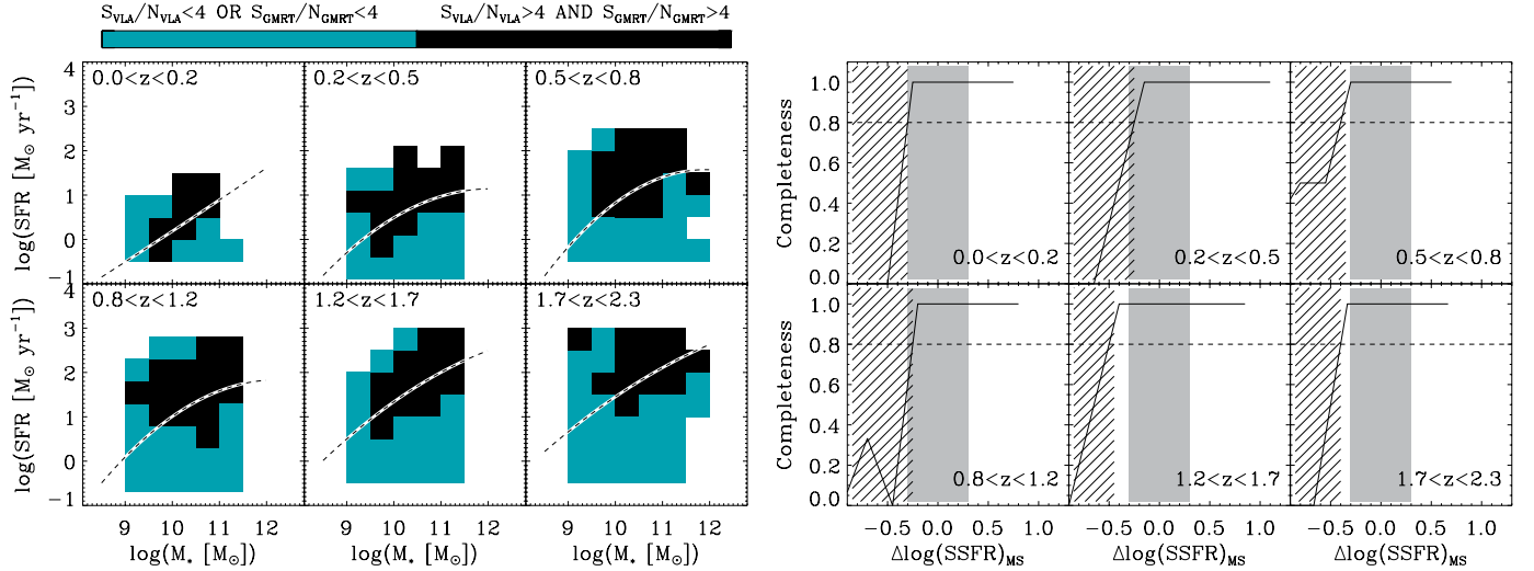
Fig. 3. Left: SFR- M_* bins with accurate \alpha_{610MHz}^{1.4GHz} estimates from our stacking analysis. Estimates are considered accurate if S_{1.4GHz}/N_{1.4GHz} > 4 (i.e. signal, S , over noise, N , ratio) and S_{610MHz}/N_{610MHz} > 4 . Short-dashed lines on a white background show the MS of star formation. Right: fraction of SFR- M_* bins with M_* > 10^{10} M_\odot and with accurate \alpha_{610MHz}^{1.4GHz} estimates as function of their \Delta \log(SSFR)_{MS} . Horizontal dashed lines represent the 80% completeness limits. Hatched areas represent the regions of parameter space affected by incompleteness, i.e. where less than 80% of our SFR- M_* bins have accurate \alpha_{610MHz}^{1.4GHz} estimates. Shaded regions show the location and dispersion of the MS of star formation.
