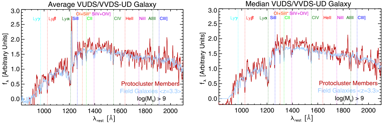
Fig. 15. Left: rest-frame mean “coadded” VUDS spectra of all spectral members of ClJ0227-0421 with \log(M_s) > 9 plotted against that of the field galaxy sample. All type-1 AGN hosts are removed from both samples. Important spectral features are noted. The two spectra exhibit remarkably similar properties. Subtle differences do exist; the average protocluster galaxy appears to have slightly stronger emission features (Ly \alpha , HeII, and CIII) and a steeper rest-frame NUV continuum slope. Right: median “coadded” VUDS spectra of the same two samples shown in the left panel . The major difference between the median spectra and the mean spectra plotted in the left panel is the enormous decrease in the strength of the Ly \alpha line, which is a reflection of the fact that most galaxies do not emit Ly \alpha at these redshifts. In the median spectrum, the Ly \alpha emission is roughly equivalent amongst the field galaxies and the protocluster members, owing to the similar fractional contribution of LAEs to both samples (see text). The differences in the median and mean spectra suggest that, though the galaxies in the protocluster emit Ly \alpha roughly as frequently as the general field population, those galaxies which do emit Ly \alpha in the protocluster are doing so more profusely.
