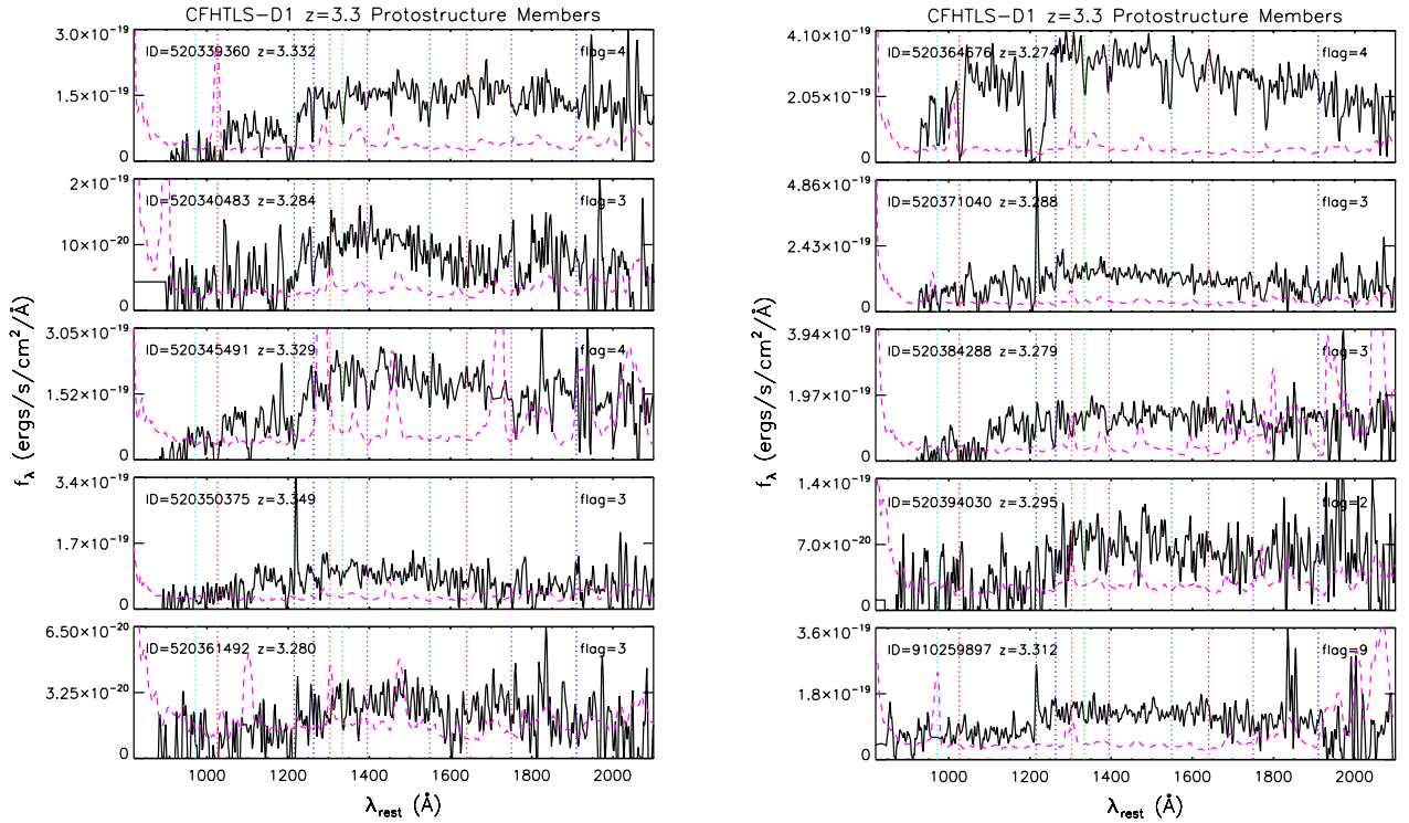
Fig. 7. Mosaic of the one-dimensional rest-frame VIMOS spectra of nine spectral members of Cl J0227-0421. Also plotted in the bottom right hand panel (ID = 910259897) is the only member with a less secure spectroscopic redshift that exhibits a strong emission line in its spectrum. In this case we presume the line to be Ly \alpha , though this galaxy does not enter any of our analysis and is presented here and elsewhere only for illustrative purposes. The meanings of all lines are the same as in Fig. 6.
