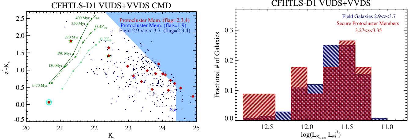
Fig. 9. Left: observed-frame CFHTLS/WIRDS color–magnitude diagram (CMD). Members of ClJ0227-0421 with secure spectroscopic redshifts are shown as red diamonds, those with less secure spectroscopic redshifts are shown as blue Xs. The meanings of the green star and cyan circle are the same as those in Fig. 3. All galaxies in the entire CFHTLS-D1 field with secure spectroscopic redshifts 2.9 < z_{\text{spec}} < 3.7 that do not reside in the bounds of ClJ0227-0421 (i.e., “field galaxies”, see Sect. 4.1) are plotted as small navy points. The light blue-shaded region indicates the region of this phase space not probed to the 5\sigma point-source completeness limits of the CFHTLS/WIRDS imaging. Model tracks for a z = 3.3 L^* galaxy with three different stellar metallicities are overplotted (see Sect. 4.1.2). Several galaxies which are extremely bright in the K_s band, including two of the four brightest galaxies in the entire spectroscopic sample over this redshift range, are members of the protocluster. Right: fractional distribution of observed-frame K_s -band luminosities in the protocluster and field samples. Only those protocluster members with secure spectroscopic redshifts and only those galaxies lying outside of the blue shaded region in the left panel are plotted. Though a large fraction of the protocluster member galaxies have relatively normal K_s -band luminosities with respect to the general field population, the percentage of bright ( \log(L_{K_s}) \gtrsim 12.0 ) galaxies residing in ClJ0227-0421 is nearly double that of the field.
