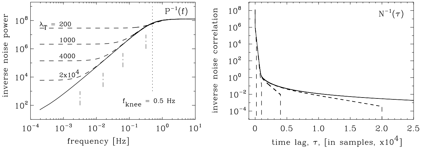
Fig. D.1. Effects of imposing band-diagonality on the inverse noise correlation matrix, N^{-1} , right panel , and its consequences for the inverse noise power spectrum, P(f) , left panel . The apodization kernel used here is defined in Eq. (D.4). The right panel shows a first row of the matrix, which is assumed to be Toeplitz. In both panels , solid lines show the result derived for the noise spectrum as in Eq. (19) without applying any apodization. Dashed lines show the results when the apodization is applied with the kernel length, \lambda_T , assuming values, 10^4 , 2000, 500 and 100, as shown bottom-up, in the left panel , and right-to-left in the right panel . Dash-dot-dash lines in the left panel show the characteristic frequency at which the apodized spectrum deflects from the original one for each apodization length. This frequency is given by f_{\text{defl}} = 1/\pi\lambda_T t_{\text{samp}} .
