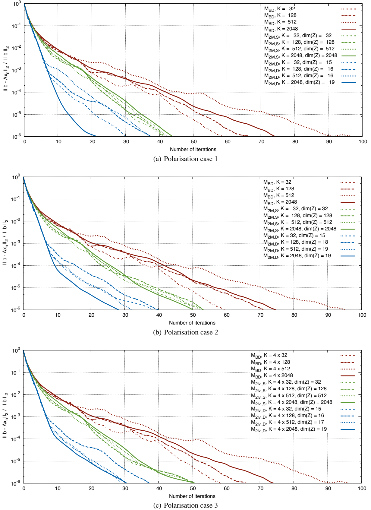
Fig. 3. Convergence of the preconditioned CG solver applied to the simulated data, as described in Sect. 5.2. Different line styles correspond to different sizes of the problem, while different colours correspond to the three different types of preconditioners: red for the standard block preconditioner \mathbf{M}_{\text{BD}} , and green and blue for the two-level preconditioners, \mathbf{M}_{2\text{lvl},\text{S}} and \mathbf{M}_{2\text{lvl},\text{D}} , respectively. In the legend, K corresponds to the number of stationary intervals in the time domain data and \dim(\mathbf{Z}) denotes the number of columns in the deflation subspace operator, \mathbf{Z} . For the a posteriori preconditioner, \mathbf{M}_{(2\text{lvl},\text{D})} , \dim(\mathbf{Z}) is the number of eigenvalues, which fulfill the condition \text{Re}|\lambda_i| < \epsilon_{\text{tol}} = 0.2 .
