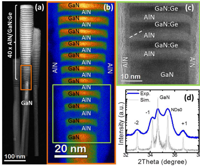
FIG. 1. (Color online) (a) HAADF STEM image of the GaN/AiN NW heterostructures. The AlN barriers (darker) and GaN disks (brighter) have nominal thicknesses of 4 nm. (b) Zoom into the squared region in (a) displayed in temperature color code. (c) HRTEM image of the first three GaN:Ge disks (near the GaN stem). (d) HRXRD \omega - 2\theta scan around the (0002) reflection of sample N3, together with a simulation. The simulation is down shifted for clarity.
