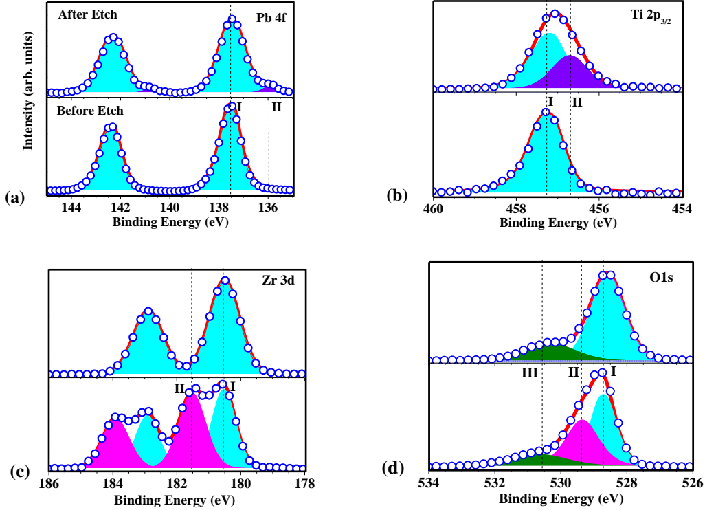
Figure 6: PZT10 a) Pb 4 f ; b) Ti 2 p 3/2 c) Zr 3 d and d) O 1 s core level spectra before and after ion beam etching. Open circles are the experimental points, continuous (red) lines the best fit. Color coding of the core level components as for Fig. 3.
