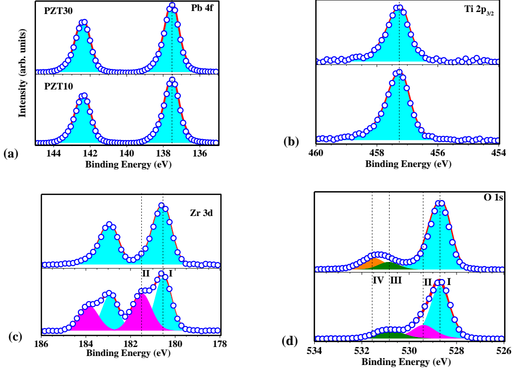
Figure 3: XPS core level spectra for a) Pb 4 f ; b) Ti 2 p 3/2 c) Zr 3 d and d) O 1 s . Open circles are the experimental points, red lines the best fit, colored peaks the different components. In each panel, the upper (lower) spectrum is that of PZT30 (PZT10). The main peak I (light gray, turquoise online) is the perovskite structure; gray peak II (magenta online) surface phase and low intensity, peaks III and IV (green and orange online) surface contaminations.
