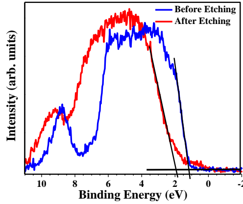
Figure 5: Valence band maxima of PZT 10 before (blue) and after IBE (red).
