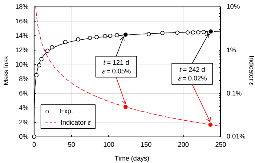
Figure 1. Illustration of the criterion \varepsilon \leq 0.05\% for the CEM I paste kept at 80^\circ\text{C} and 76% RH (in this example A = -16.04\% and B = 1.522 d^{0.5} ). Note the log-scale for the indicator \varepsilon .
