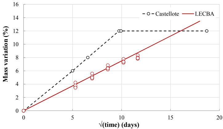
Figure 4: Mass variation of CEM I samples during accelerated carbonation test at 3% \text{CO}_2 content (22°C, 65% RH) (dotted line) [23] – Mass variation of CEM I samples during accelerated test, in LECBA, at 3% \text{CO}_2 content (25°C, 55% RH) (straight line)
