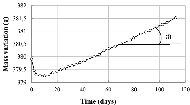
Figure 7: Cup mass evolution vs. time for a 33% (RH 1 )-50% (RH 2 ) RH range at 20°C [11]
