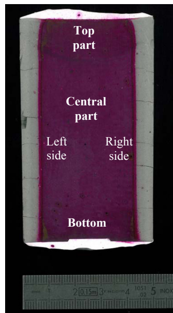
Figure 1: Degradation profile of CEM I paste sample after 1 month in ammonium nitrate (6M) at ambient temperature
