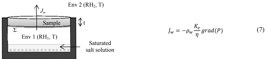
Figure 6: Sketch of the cup-method test
