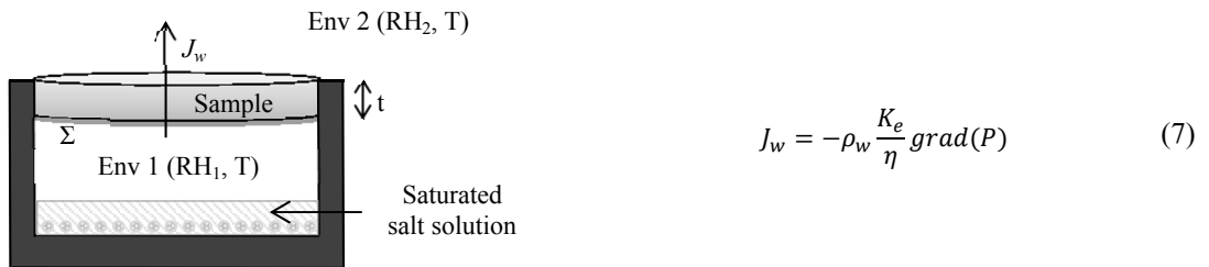
Figure 6: Sketch of the cup-method test
