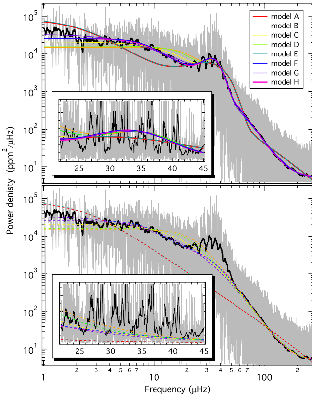
Fig. 4. Raw (grey) and heavily smoothed (black) power density spectrum of KIC 7949599. Over-plotted in colour are the best fits model with (top panel) and without (bottom panel) the Gaussian component. Note that model A and E and model F and G effectively overlap. The inserts show enlarged sections around \nu_{\max} .
