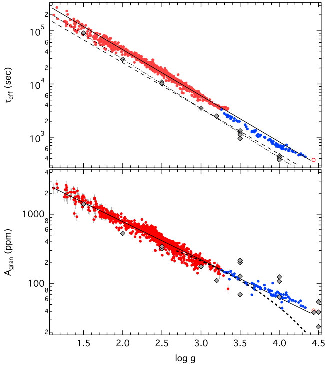
Fig. 9. Characteristic timescale \tau_{\text{eff}} (top) and intensity fluctuations A_{\text{gran}} (bottom) as a function of \log g for our sample of LC (red) and SC (blue) stars. Solid lines correspond to power law fits. The dashed line in the top panel corresponds to a power law fit to effective timescales obtained from 3D simulations (Mathur et al. 2011). Diamond symbols indicate values obtained from the granulation spectrum of 3D hydrodynamical models (Samadi et al. 2013b) and the dotted line corresponds to a power law fit to these models. The dashed line in the bottom panel shows the relation between the 8 h-flicker amplitude and \log g .
