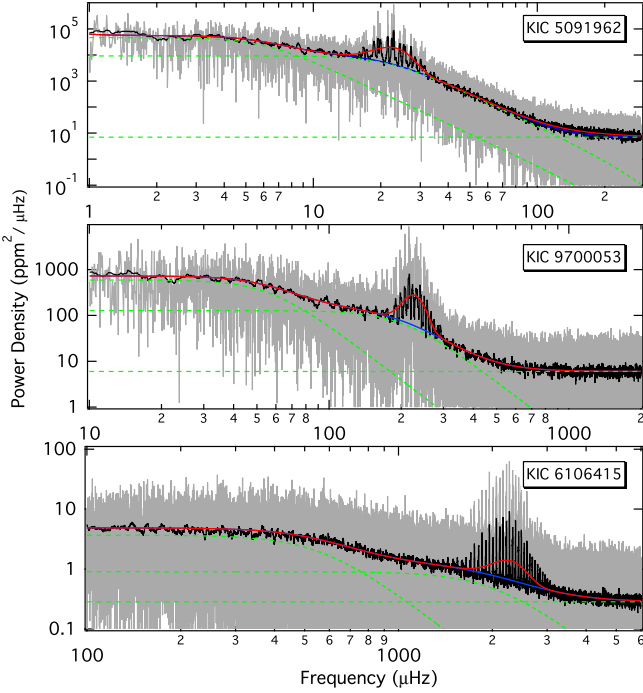
Fig. 7. Power density spectra of three typical stars with \nu_{\max} \approx 22 , 220, and 2200 \mu\text{Hz} , respectively, showing that all timescales and amplitudes (granulation as well as pulsation) scale simultaneously. Grey and black lines indicate the raw and heavily smoothed spectrum, respectively. The global fit is shown with (red) and without (blue) the Gaussian component. Green lines indicate the individual background and white noise components of the fit.
