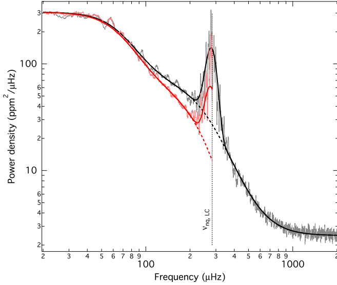
Fig. 3. Heavily smoothed ( 5\mu\text{Hz} boxcar filter) power density spectrum of the about 540 and 1000 day-long SC (grey line) and LC Kepler time series (light-red line), respectively, of KIC 5596656. The black lines correspond to the best-fit model for the SC data with (full line) and without (dashed line) the Gaussian component. The red lines indicate the SC model corrected for the amplitude suppression due to the longer sampling. The vertical dotted line marks the Nyquist frequency for the LC sampling.
