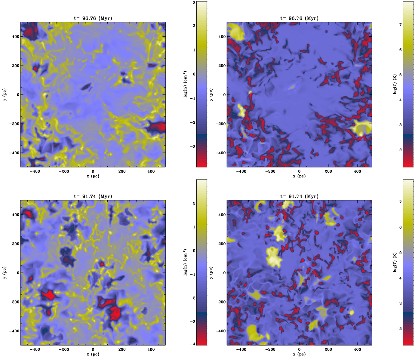
Fig. 9. Density (left column) and temperature (right column) fields in the equatorial plane for the MHD run C1 (upper panel) and the hydrodynamical run C2 (lower panels). The figures illustrate the multi-phase nature of the interstellar medium. Most of the volume is filled by warm neutral gas with temperature of about 8000 K. A tiny fraction is occupied by the hot phase at temperature larger than 10^6 K.
