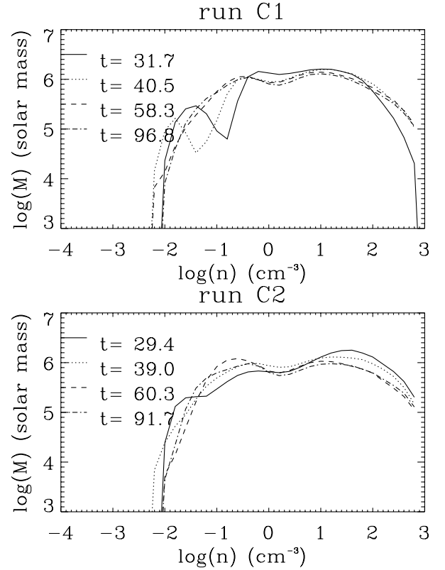
Fig. 7. Probability density function for MHD run C1 ( upper panel ) and hydrodynamical run C2 ( lower panel ). The small dip at n \approx 2\text{--}3\text{ cm}^{-3} corresponds to the thermally unstable regime, which persists in spite of the strong turbulence. The two peaks correspond to the WNM and CNM phases.
