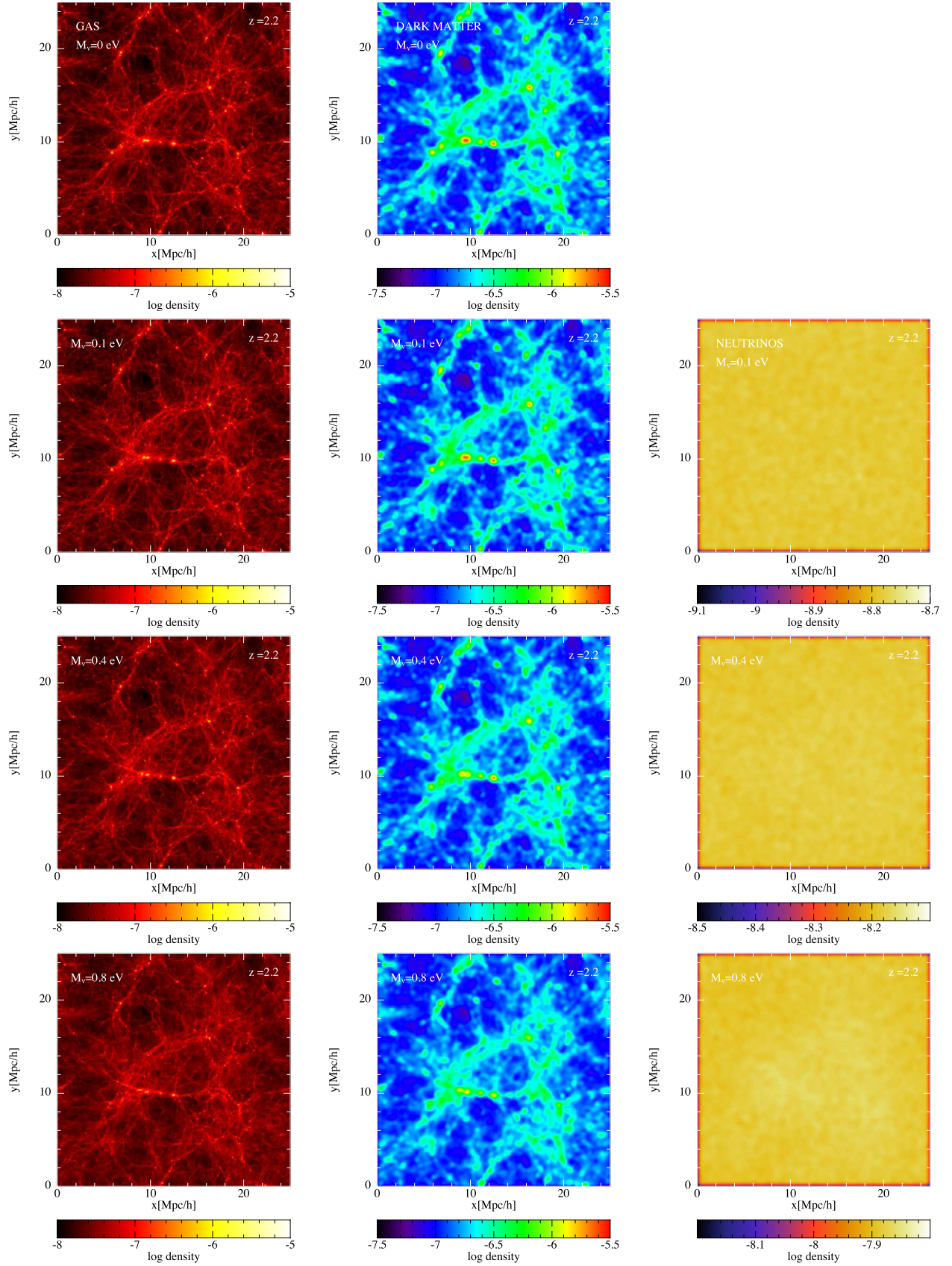
Fig. 4. Visual examples of snapshots at z = 2.2 from simulations with a box size of 25 h^{-1} Mpc and a resolution of N_p = 192^3 particles per type. The upper top panels are full projections of the density field in the x and y directions across z from our best-guess reference simulation without massive neutrinos (but with a massless neutrino component), while in descending order the other panels are for M_\nu = 0.1, 0.4 , and 0.8 eV. Gas ( left panels ), dark matter ( central panels ), and neutrino ( right panels ) components – when present – are shown. The axis scales are in h^{-1} Mpc. The various plots are smoothed with a cubic spline kernel, and both the DM and neutrino components are treated in the same way as the gas. See the text for more details.
