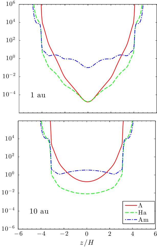
Fig. 2. Ohmic ( \Lambda ; Eq. (15)), Hall ( Ha ; Eq. (16)), and ambipolar ( Am ; Eq. (17)) Elsasser numbers in the initial state versus height z at 1 au (top) and 10 au (bottom), assuming a constant vertical magnetic field with \beta_0 = 10^5 .
