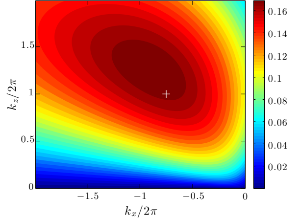
Fig. B.2. Growth rate of the ambipolar-MRI for B_{x0} = 0.025 and B_{y0} = 0.1 as a function of the horizontal and vertical wavenumbers, k_x and k_z . The largest growth rate available in the simulation obtains for (k_x, k_z) = 2\pi \times (-0.75, 1) (white cross).
