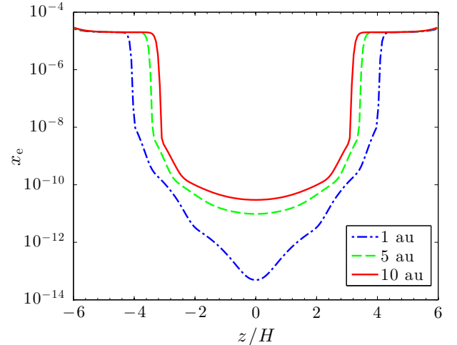
Fig. 1. Ionisation fraction x_e versus height z at 1, 5, and 10 au.
