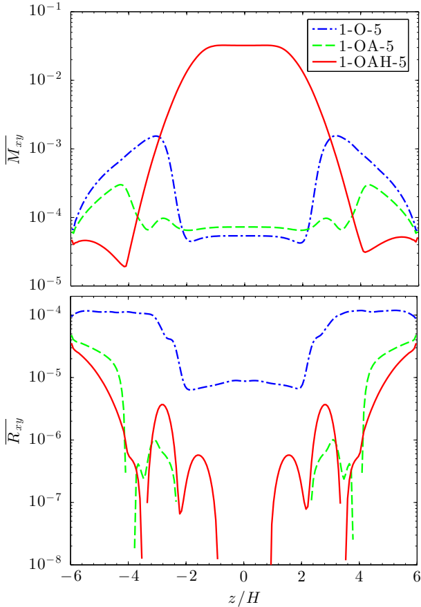
Fig. 10. Horizontally averaged Maxwell ( top ) and Reynolds ( bottom ) stress versus height z , averaged over 700 \Omega^{-1} , from runs 1-O-5 (dash-dotted), 1-OA-5 (dashed), and 1-OAH-5 (solid).
