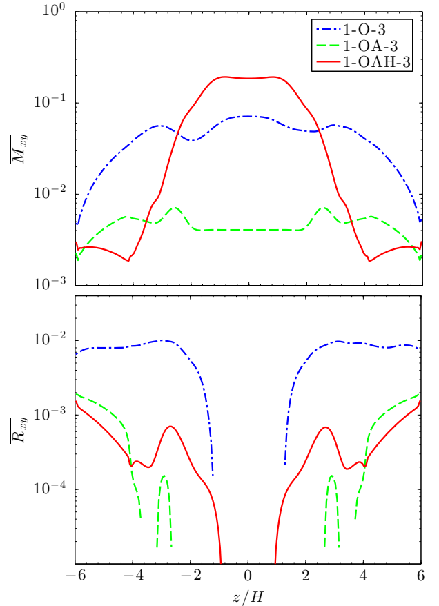
Fig. 12. Horizontally and temporally averaged Maxwell ( top ) and Reynolds ( bottom ) stress versus height z for runs 1-O-3 (dash-dotted), 1-OA-3 (dashed), and 1-OAH-3 (solid).
