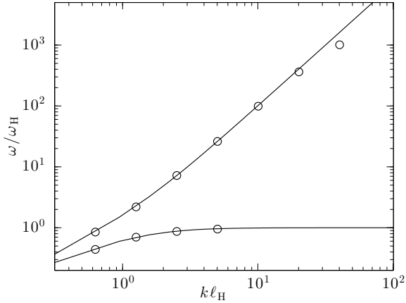
Fig. A.1. Dispersion relation for whistler waves. Black line: analytical prediction; circles: eigenfrequencies measured in PLUTO using our implementation of the Hall effect.
