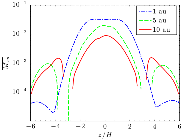
Fig. 13. Horizontally averaged Maxwell stress versus height z , averaged over 700 \Omega^{-1} , from runs 1-OAH-5 (dash-dotted), 5-OAH-5 (dashed), and 10-OAH-5 (plain line).
