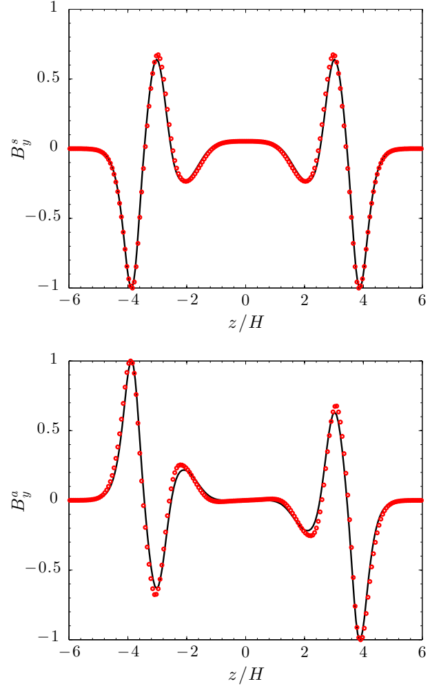
Fig. 4. Comparison of B_y(z) from the simulation (red circles) and from the linear calculation (black line), which include Ohmic and Hall diffusion computed at 1 au with \beta_0 = 10^5 . Top: n = 1 eigenmode and symmetric component of B_y(z) . Bottom: n = 2 eigenmode and antisymmetric component of B_y(z) .
