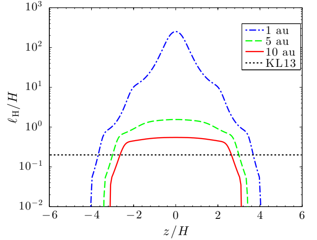
Fig. 3. Hall lengthscale \ell_H (Eq. (18)) versus height z at 1, 5, and 10 au. The dotted line denotes the threshold above which saturation via zonal magnetic fields occurs in unstratified simulations with net vertical magnetic flux (KL13).
