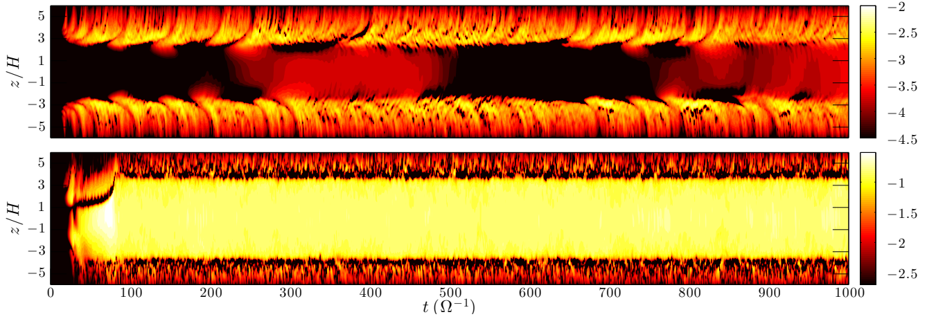
Fig. 6. Space–time diagram of the logarithm of the horizontally averaged Maxwell stress, \log\langle -B_x B_y \rangle , in the Ohmic (1-O-5; top ) and Ohmic-Hall (1-OH-5; bottom ) runs.
