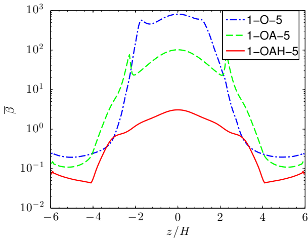
Fig. 11. Horizontally averaged turbulent plasma \beta versus height z , averaged over 700 \Omega^{-1} , from runs 1-O-5 (dash-dotted), 1-OA-5 (dashed), and 1-OAH-5 (solid).
