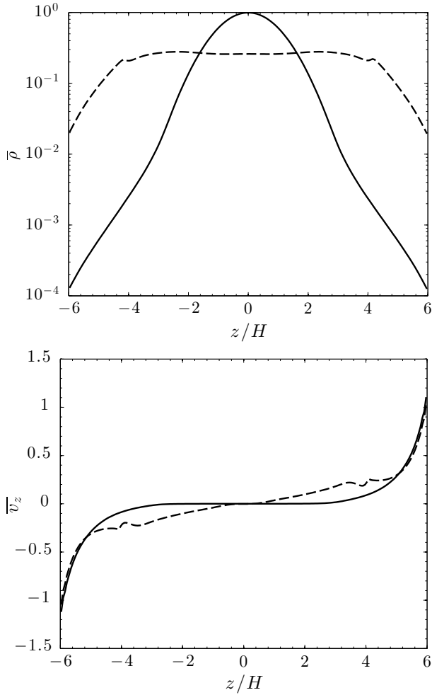
Fig. 7. Horizontally averaged density profile \bar{\rho} (top) and vertical velocity \bar{v}_z (bottom) versus height z , averaged over \approx 140 orbits, from runs 1-O-5 (solid line) and 1-OH-5 (dashed line).
