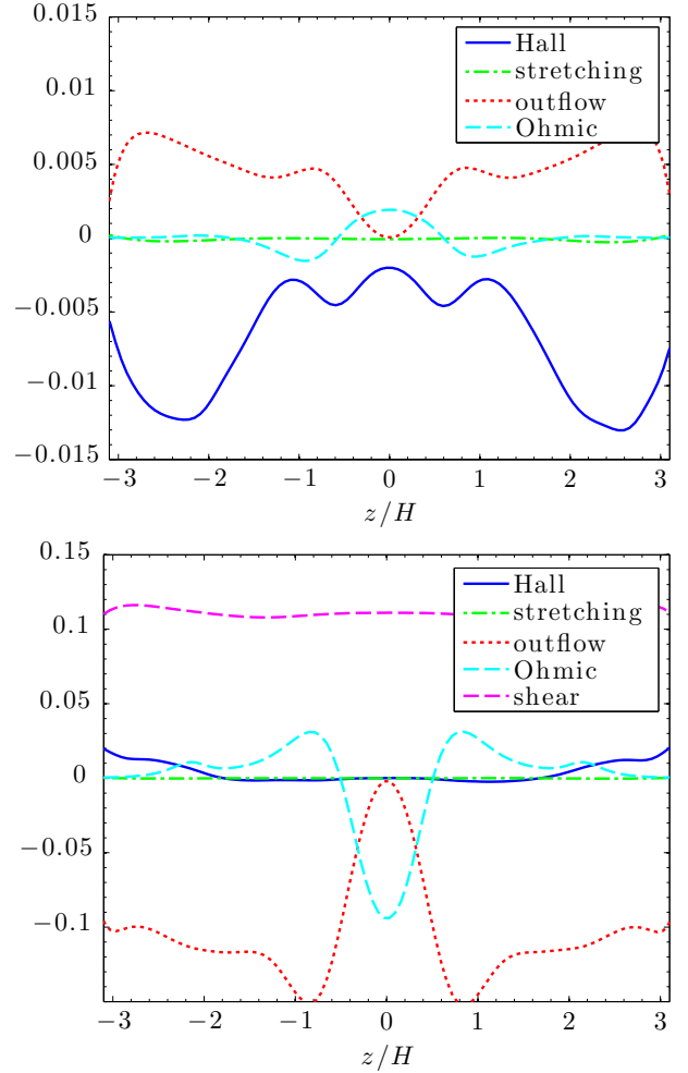
Fig. 8. Contributions in run 1-OH-5 to the right-hand side of the horizontally averaged induction equation deduced from Eqs. (20a; top) and (20b; bottom).
