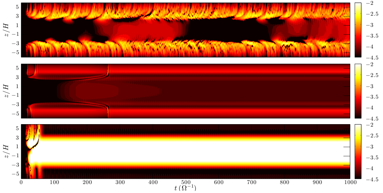
Fig. 9. Space–time evolution of the logarithm of the horizontally-averaged magnetic stress, \log\langle M_{xy} \rangle , in the Ohmic (1-O-5; top ), Ohmic-ambipolar (1-OA-5; middle ), and Ohmic-ambipolar-Hall (1-OHA-5; bottom ) runs.
