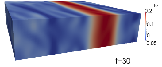
Fig. A.2. Snapshot of B_z in our unstratified Hall-MRI run at t = 30 . The flow exhibits a zonal-field structure similar to that discovered by KL13.
