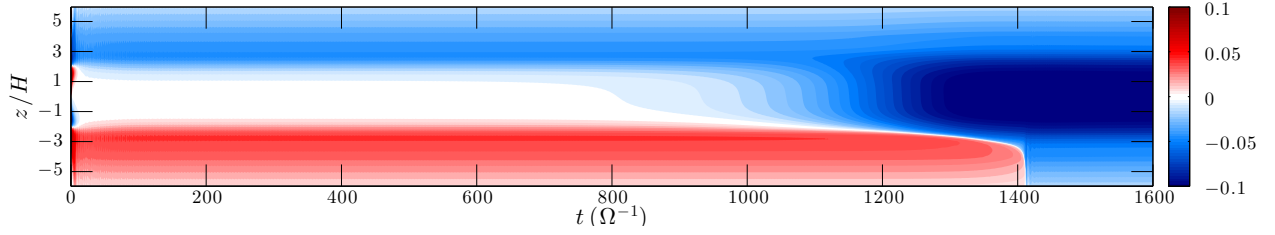
Fig. 14. Space–time evolution of the horizontally averaged azimuthal magnetic field, \langle B_y \rangle , as a function of time in run 1-OA-5-e. The run starts with odd symmetry for the azimuthal field. At t \approx 1000 \Omega^{-1} a current layer forms and is ejected at t = 1410 \Omega^{-1} , leaving an azimuthal field with even symmetry.
