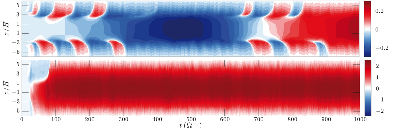
Fig. 5. Space–time diagram of the horizontally averaged azimuthal magnetic field, \langle B_y \rangle , in the Ohmic (1-O-5; top ) and Ohmic-Hall (1-OH-5; bottom ) runs.
