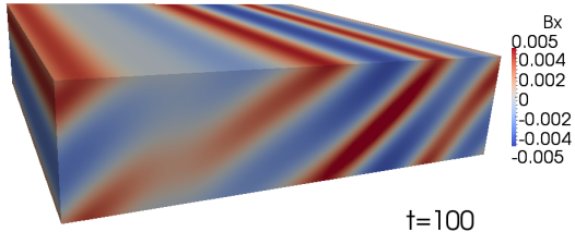
Fig. B.1. Snapshot of B_x in our ambipolar-MRI test simulation at t = 100 , just before saturation. The oblique nature of MRI channel mode, as predicted by Kunz & Balbus (2004), is evident.
