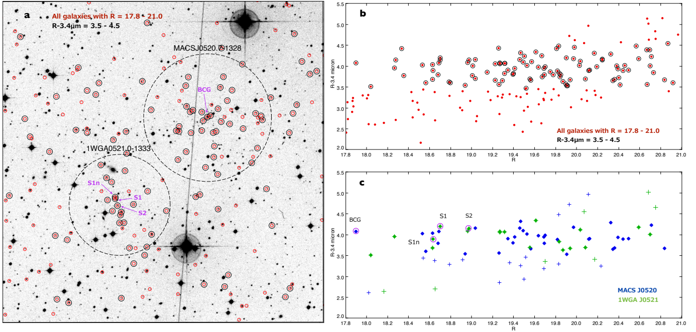
Fig. 5. a) DSS-R image of the \sim 19' \times 19' area around M0520 (same as in Fig. 1, Right panel ); dashed circles have radii r_{500} and are centred on the X-ray centre of each cluster. The red small circles mark the galaxies selected in the range R = 17.8-21.0 ; the large black circles show only those galaxies within the range of colours R - 3.4 \mu\text{m} = 3.5-4.5 . b) R - 3.4 \mu\text{m} CMD of the galaxies within the \sim 19' \times 19' area as in panel a) red and black circles as in panel a) . c) R - 3.4 \mu\text{m} CMD of the galaxies within the dashed circles in panel a) the crosses are all the galaxies in the range R = 17.8-21.0 , the filled dots are the colour-selected once ( R - 3.4 \mu\text{m} = 3.5-4.5 ). The BCG of M0520 and the optical counterparts of radio sources S1 and S2 are marked by magenta circles (they are also highlighted by magenta arrows in panel a) , for clarity).
