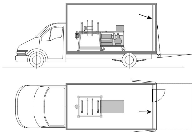
FIG. 3. Side and top views of the installation inside the van. The arrows indicate the plywood wall.
