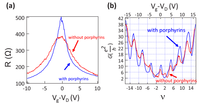
FIG. 3. Improvement of the sample quality after porphyrins deposition (Pd/Nb sample). (a) Zero magnetic field gate voltage sweep of two wire resistance at 4.2 K, before (red) and after (blue) deposition of Pt-porphyrins. The origin is taken at the Dirac point V_D for both curves. The sharper curve with a higher Dirac peak demonstrates that the sample quality has improved thanks to porphyrin coating, with a mobility increase of 20%. (b) Two-wire measurement of the resistance in the quantum Hall regime, at 100 mK and in a perpendicular magnetic field of B = 5 T (for which the Nb electrodes are nonsuperconducting), before (red curve) and after (blue curve) grafting. The gate voltage is expressed in terms of the filling factor \nu = n_c \phi_0 / B , with the charge density n_c computed assuming that only the backgate charges the graphene. The Hall plateaus (visible even in a two wire measurement) are better defined, confirming the higher sample quality. The gate voltage position of the plateaus is unchanged, demonstrating that the charge transfer between porphyrins and graphene is gate independent, and fixed at low temperature.
