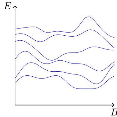
Chaotic billiard
