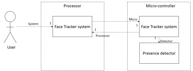
Figure 10: Face Tracker system design
