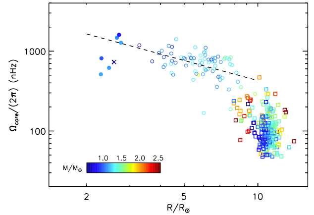
Fig. 14. Core rotation rate as a function of the stellar radius. The open symbols correspond to the stars studied by Mosser et al. (2012b, circles: RGB stars, squares: clump stars). The filled symbols indicate the stars that were studied in this paper, and the cross corresponds to the young giant KIC 7341231 studied by D12.
