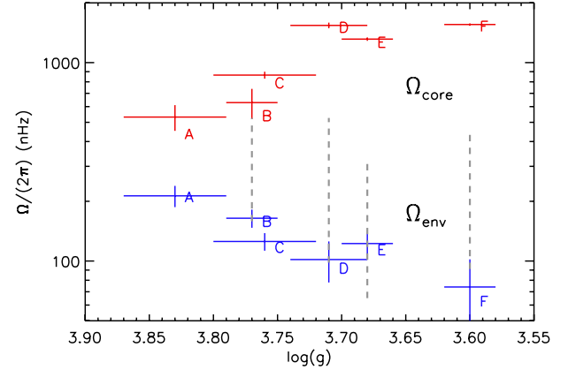
Fig. 13. Core (red symbols) and envelope (blue symbols) rotation rates obtained with the OLA method (see Sects. 6.2.1 and 6.2.2) plotted as a function of the surface gravity. The letter corresponding to each star is specified. The dashed gray lines correspond to the range of surface rotation rates predicted by van Saders & Pinsonneault (2013) for the stars that lie in the range of parameters that they considered. The horizontal and vertical lines indicate 1\sigma error-bars.
