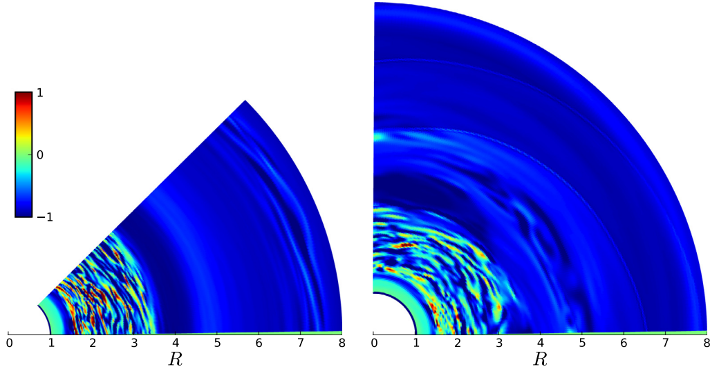
Fig. 12. Vortensity ((V - V_{\text{init}})/V_{\text{init}}) map in the disk (R, \phi) plane. The left panel shows the midplane vortensity in the \sigma_{\text{hot}} simulation with the small azimuthal extend. The right panel shows the midplane vortensity in the \sigma_{\text{hot}} simulation which has \phi \in [0, \pi/2] .
