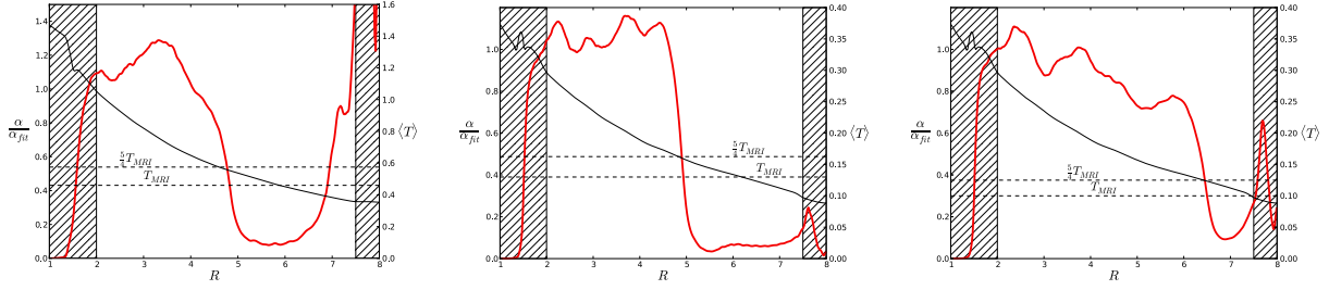
Fig. 11. \alpha profiles averaged over 100 orbits after the fronts have reached their final position ( \alpha values are listed on the left axis). Left panel: \sigma_{\text{hot}} simulation which T_{\text{MRI}} = 0.46 . Middle and right panels: \sigma_{\text{cold}} simulation which T_{\text{MRI}} = 0.1 and T_{\text{MRI}} = 0.13 respectively. The black plain lines remind the temperature profiles from ideal cases. Black dashed lines show the threshold value T_{\text{MRI}} and 5/4 T_{\text{MRI}} . The temperature values are listed on the right axis.
