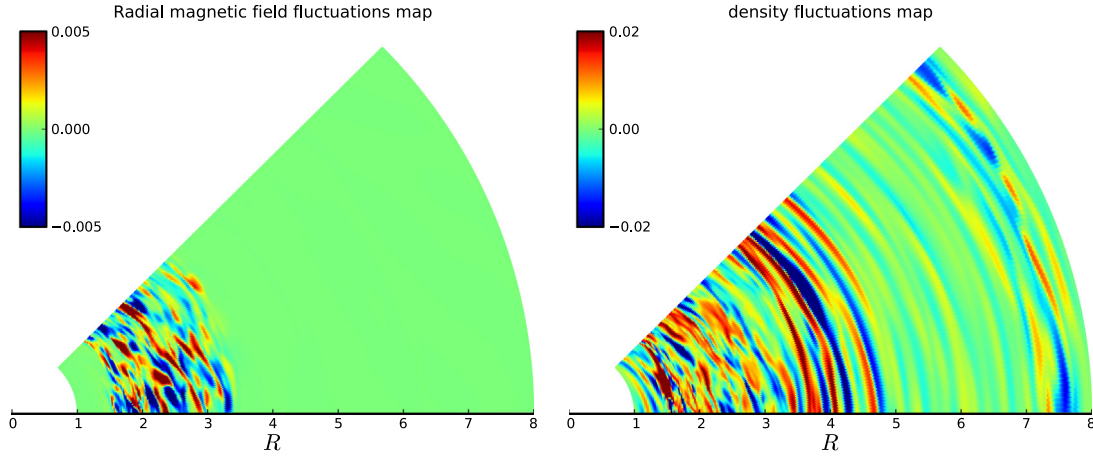
Fig. 5. z = 0 planar maps of radial magnetic fields fluctuation (on the left) and density fluctuations (right plot) from the \sigma_{\text{hot}} simulation at t = 900 + \tau_{\text{cool}} (R = 7R_0) .
