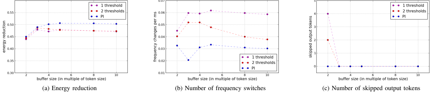
Fig. 9. Comparison of 3 controllers for medium QoS level ( 0.7 \cdot QoS_{max} ), various buffer sizes
