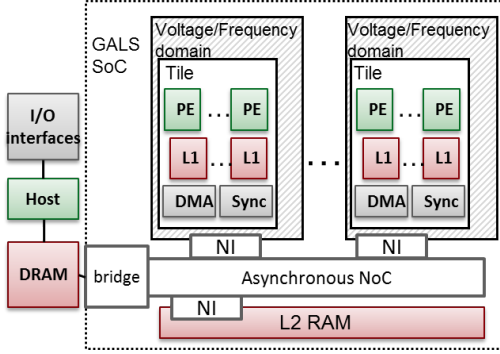
Fig. 1. Tiled SoC template
