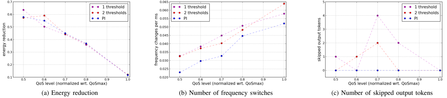
Fig. 10. Comparison of 3 controllers for small buffer size (2 · token size), various QoS levels
