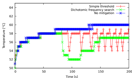
Fig. 5. Thermal execution profiles for the die center temperature (FC) for two mitigation schemes on board.
