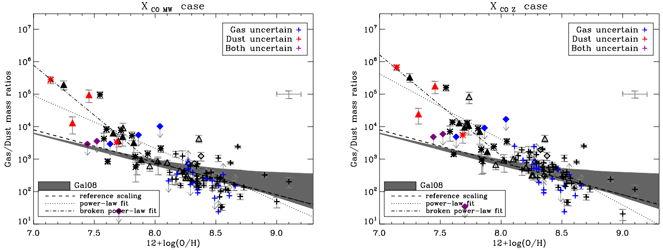
Fig. 6. G/D as a function of metallicity for the 2 values of X_{\text{CO}} : X_{\text{CO,MW}} (left) and X_{\text{CO,Z}} (right) with the chemical evolution model of Galliano et al. (2008) . The colours and symbols are the same as for Fig. 4. The dark grey stripes show the range of values from the Galliano et al. (2008) chemical evolution model. The black dashed line represents the reference scaling of the G/D with metallicity (not fit to the data). The black dotted and dash-dotted lines represent the best power-law and best broken power-law fits to the data.
