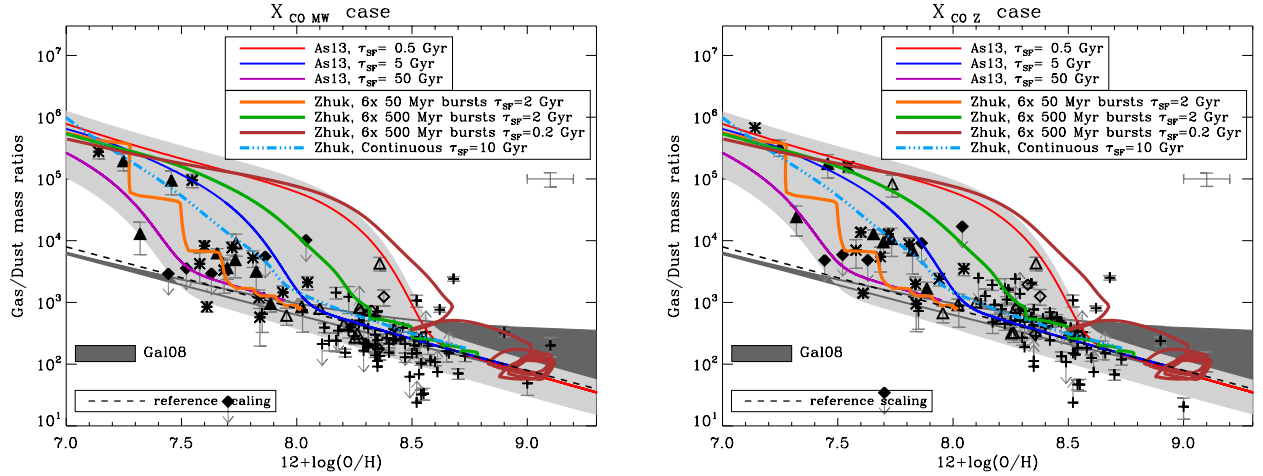
Fig. 9. G/D as a function of metallicity for the 2 values of X_{\text{CO}} : X_{\text{CO,MW}} (left) and X_{\text{CO,Z}} (right) with the three chemical evolution model considered in Sect. 4. The symbols are the same as for Fig. 4. The model ranges from Galliano et al. (2008) are delineated by the dark grey stripe. The models from Asano et al. (2013a) are shown with the red, blue and purple lines and the light grey tolerance zone. The models from Zhukovska (2014) are shown with the orange, green solid lines and cyan dash-3 dots line. The black dashed line represents the reference scaling of the G/D with metallicity (not fit to the data).
