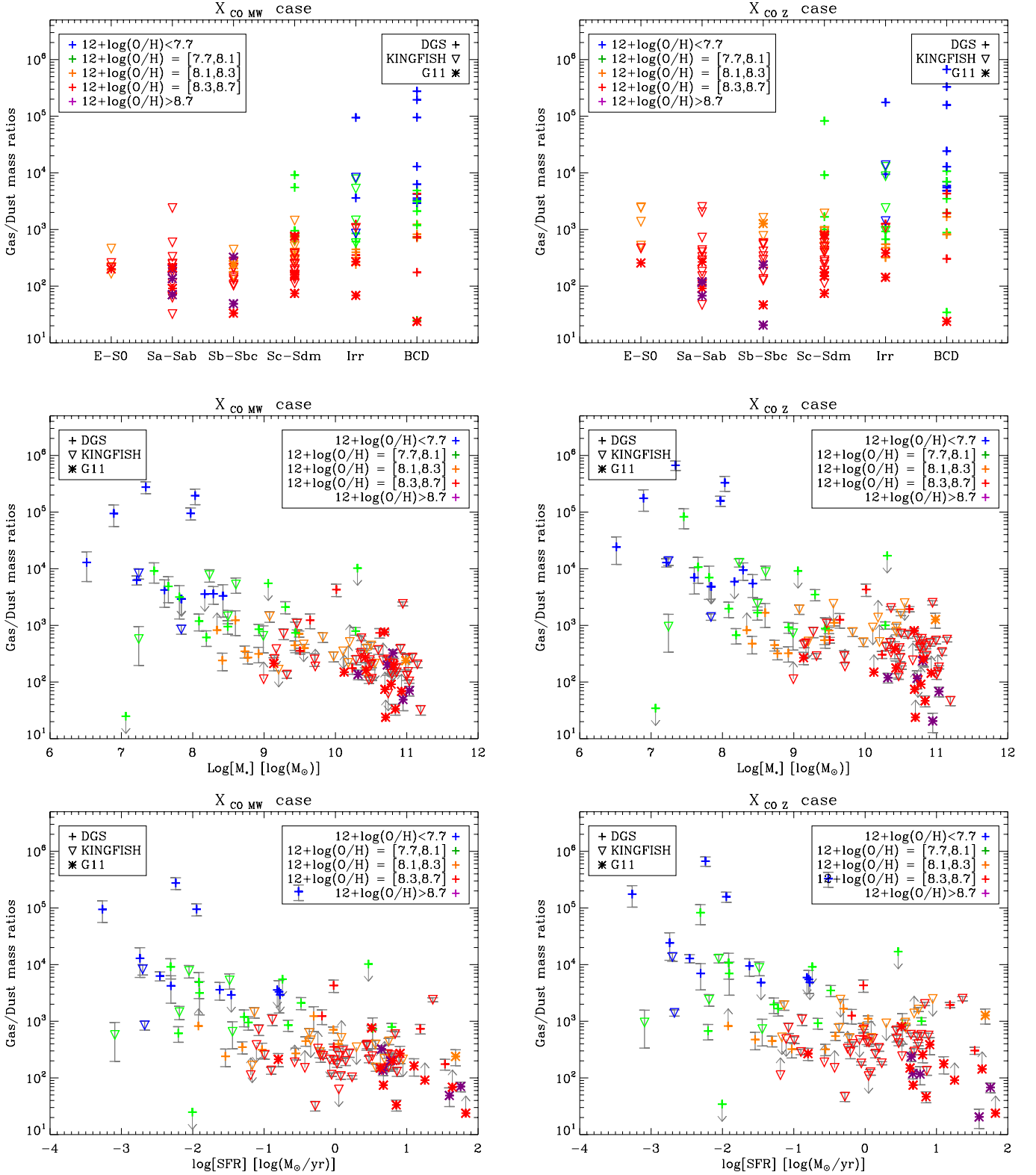
Fig. B.3. G/D as a function of morphological type ( top row ), stellar mass ( centre row ) and star formation rate ( bottom row ) for the 2 values of X_{\text{CO}} : X_{\text{CO,MW}} ( left column ) and X_{\text{CO,Z}} ( right column ). The colours code for the metallicity of the galaxies and the symbols differentiate between the three samples: DGS (crosses), KINGFISH (downward triangles) and G11 (stars).
