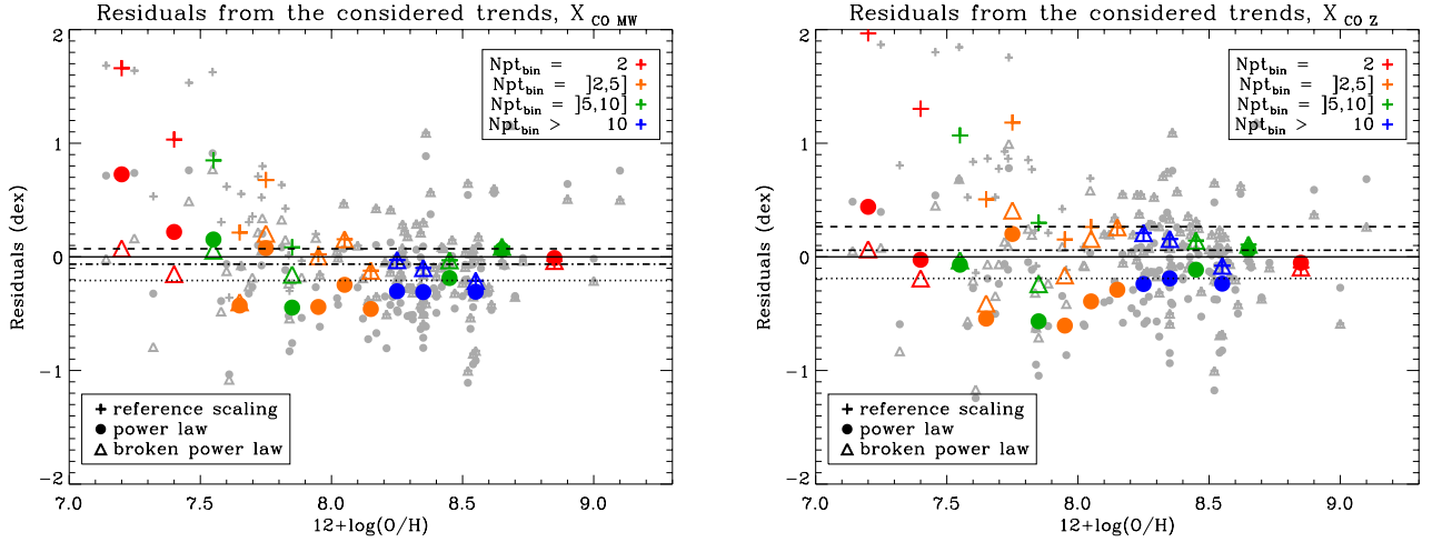
Fig. 5. Residuals (i.e., logarithmic distance) between the observed (and detected) G/D and predicted G/D from the three relations for X_{\text{CO,MW}} (left) and X_{\text{CO,Z}} (right): reference scaling of the G/D with metallicity (crosses), the best power-law fit (filled circles) and the best broken power-law fit (triangles). These residuals are shown in grey for the individual galaxies and in colour for the average residuals in each metallicity bin defined in Sect. 3.1. The colours show the number of galaxies in each bin. The mean residual for all of the observed G/D values is shown by the dashed (reference scaling), dotted (power-law fit) and dash-dotted (broken power-law fit) lines for the three relations and are reported in Table 1.
