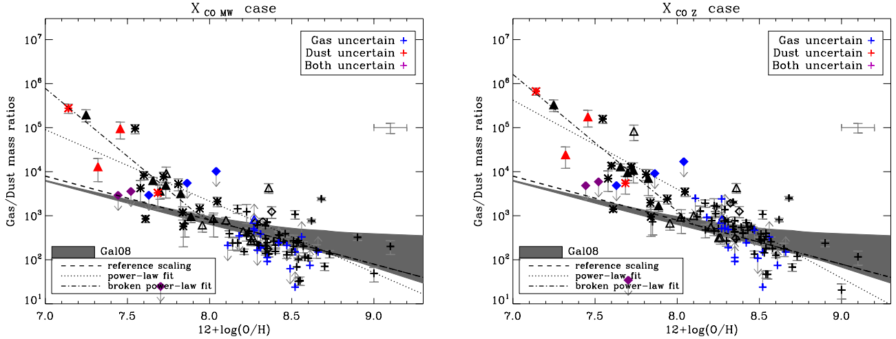
Fig. 6. G/D as a function of metallicity for the 2 values of X_{\text{CO}} : X_{\text{CO,MW}} (left) and X_{\text{CO,Z}} (right) with the chemical evolution model of Galliano et al. (2008). The colours and symbols are the same as for Fig. 4. The dark grey stripes show the range of values from the Galliano et al. (2008) chemical evolution model. The black dashed line represents the reference scaling of the G/D with metallicity (not fit to the data). The black dotted and dash-dotted lines represent the best power-law and best broken power-law fits to the data.
