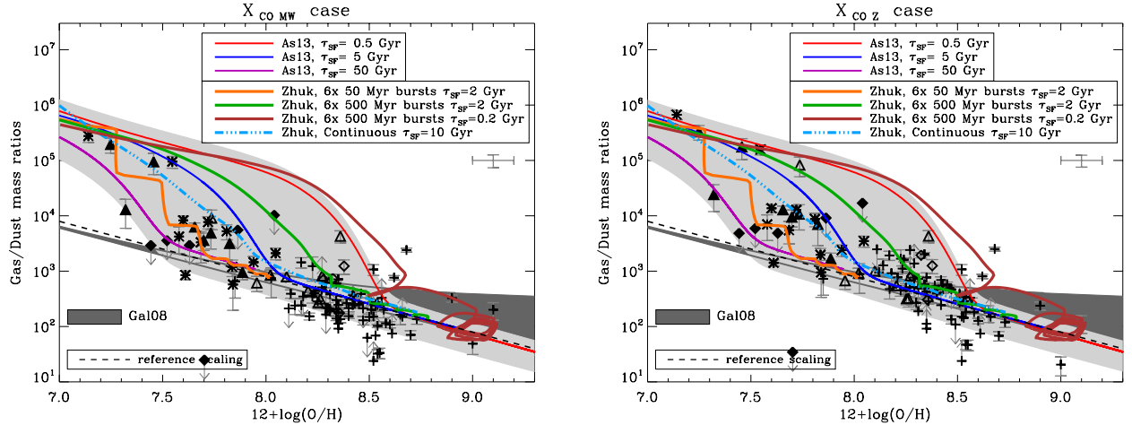
Fig. 9. G/D as a function of metallicity for the 2 values of X_{\text{CO}} : X_{\text{CO},\text{MW}} (left) and X_{\text{CO},\text{Z}} (right) with the three chemical evolution models considered in Sect. 4. The symbols are the same as for Fig. 4. The model ranges from Galliano et al. (2008) are delineated by the dark grey stripe. The models from Asano et al. (2013a) are shown with the red, blue and purple lines and the light grey tolerance zone. The models from Zhukovska (2014) are shown with the orange, green solid lines and cyan dash-3 dots line. The black dashed line represents the reference scaling of the G/D with metallicity (not fit to the data).
