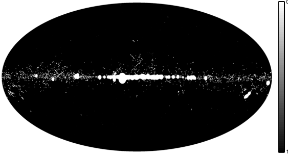
Fig. 3. Mask used for the post-processing of the compact sources. The sky coverage is equal to f_{\text{sky}} = 97\% .
