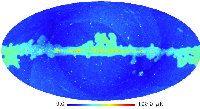
Fig. A.4. Uncertainty map of the estimated CMB map in the pixel domain.
