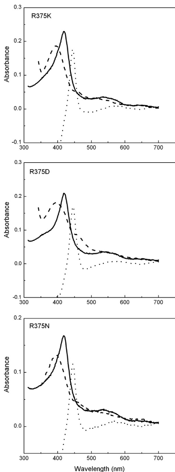
Fig. 3. Spectral properties of the R375 mutants. The spectra of proteins which were purified in the presence of 0.5 mM Arg and 3 \mu M H_4B are shown in solid lines. Dashed lines show the spectra of mutants in the presence of 10 mM Arg and 200 \mu M H_4B after incubation proteins with high concentration of Arg and H_4B overnight at 4 °C. A difference spectrum created by subtracting the spectrum of the ferric enzyme from the spectrum of the enzyme ferrous-CO complex is shown in dotted line in each panel.
