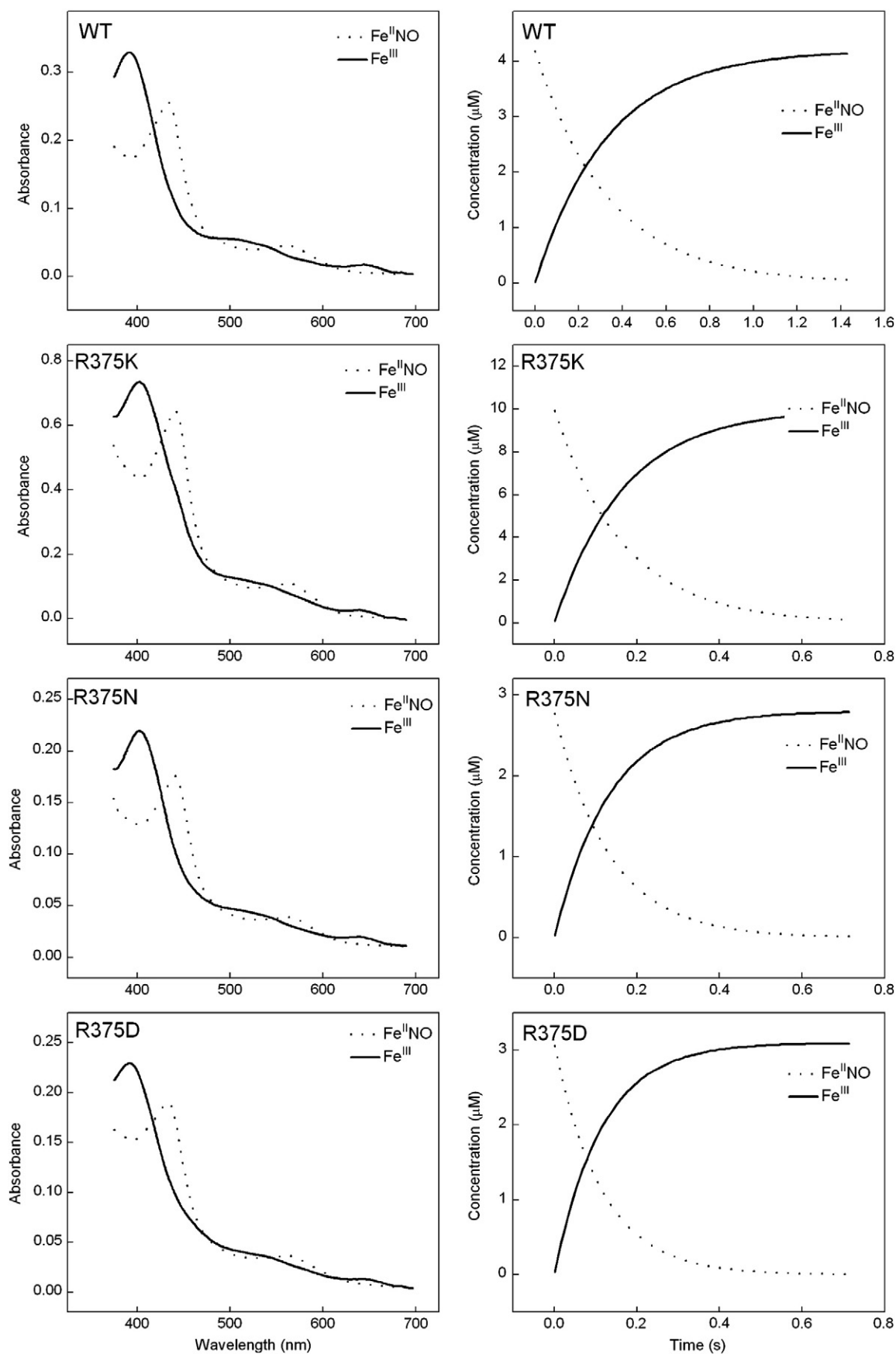
Fig. 5. Spectra and kinetics of iNOSoxy \text{Fe}^{\text{II}}/\text{NO} oxidation reactions. Anaerobic ferrous iNOSoxy proteins in the presence of Arg (10 mM) and \text{H}_4\text{B} (400 \mu\text{M} ) were titrated by small amounts of anaerobic NO-saturated buffer to form the ferrous NO complex, which was then rapid-mixed in a stopped flow spectrophotometer with air-saturated buffer at 10 °C. Left panels contain spectra of the beginning ferrous-NO and ending ferric heme species as calculated by global analysis of the spectral data, while right panels show the concentration of both species versus time after mixing. Data are representative of three experiments.
