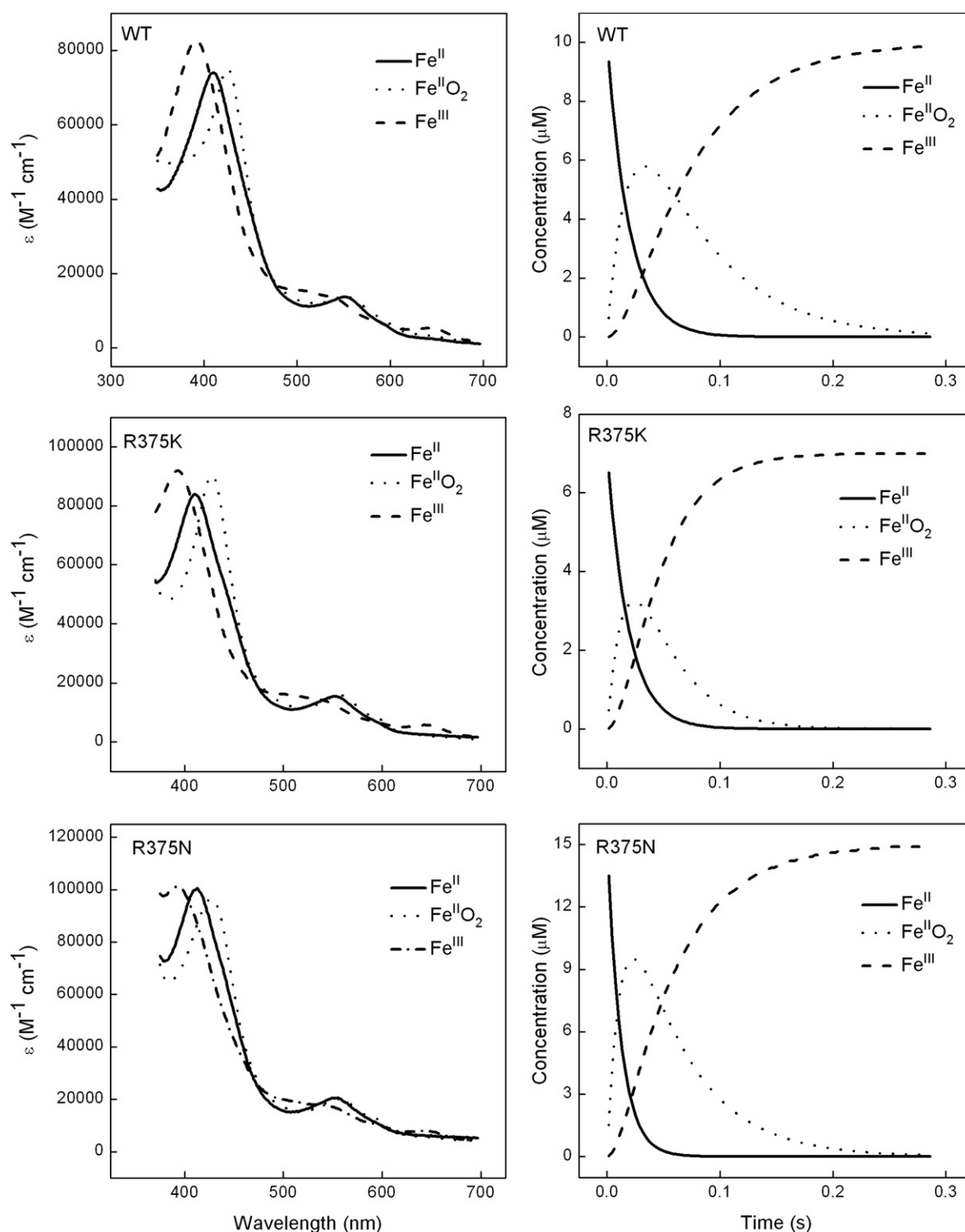
Fig. 7. Stopped-flow analysis of heme transitions and kinetics during single-turnover Arg hydroxylation catalyzed by R375K, R375N and wild type iNOSoxy. Anaerobic ferrous iNOSoxy proteins (4 \mu M) in the presence of Arg (10 mM) and H_4B (400 \mu M) were mixed in a stopped flow instrument with air-saturated buffer at 10 ^{\circ} C and diode array spectra were collected. Left panels contain three heme species that were detected during each reaction as calculated by global analysis of the spectral data, while right panels show their concentration profiles versus time after mixing. Data are representative of three similar experiments.
