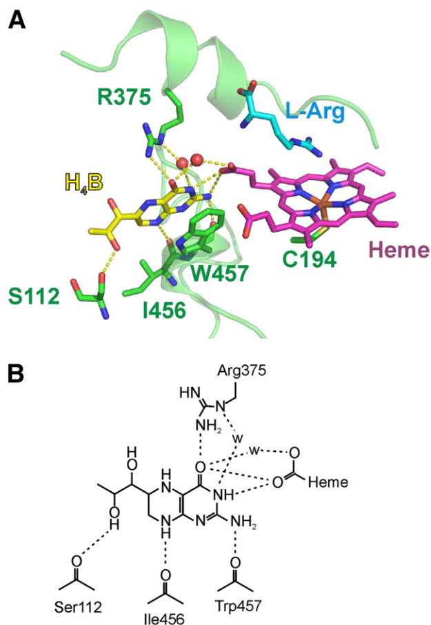
Fig. 2. Protein environment of the H 4 B cofactor. A, Interactions between H 4 B and iNOS. Several iNOS residues and the heme cofactor form a hydrogen bonding network with the H 4 B cofactor. Relevant iNOS residues are shown in green; H 4 B (yellow), Heme (pink) and the substrate L-Arg (blue) are shown as sticks. Two water molecules that mediate H-bonding interactions are shown as red spheres. The hydrogen bonding interactions are shown as yellow dashes. Note the \pi -stacking interaction between the Trp457 side chain and H 4 B. The figure was made using PyMOL ( http://www.pymol.org/ ) with the crystal structure of the mouse iNOSoxy dimer (PDB entry 1NOD [12,79]). B; Hydrogen bond interactions (dashed lines) between the H 4 B cofactor and iNOS. Ser112, Ile456 and Trp457 make H-bonds through the main chain carbonyl groups; Arg375 interacts through its side chain.
