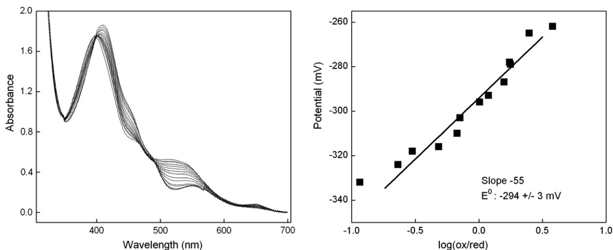
Fig. 4. Potentiometric reductive titration of R375K iNOSoxy. Left Panel shows spectra recorded during titration of the ferric enzyme in the presence of H 4 B, Arg, and mediator dyes. Right panel plots the measured potentials vs. the logarithmic ratio of ferric/ferrous heme.
