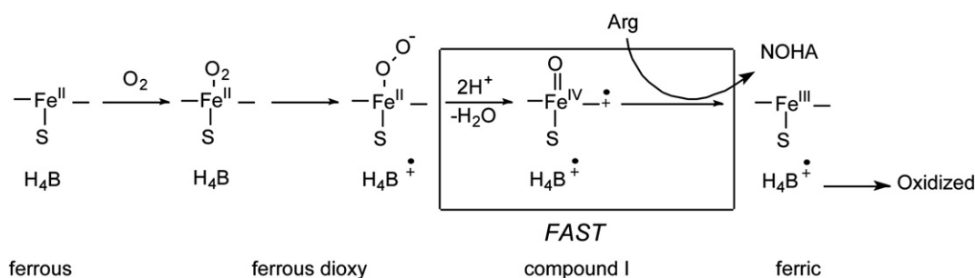
Scheme 2. Arginine hydroxylation single turnover reaction by NOS enzyme.
