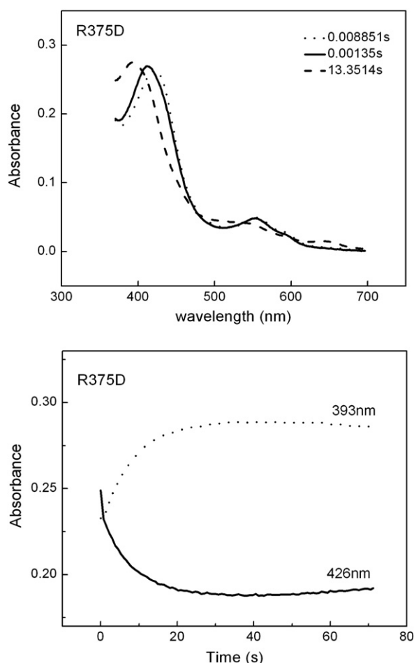
Fig. 8. Heme transitions and kinetics of R375D iNOSoxy during Arg hydroxylation single turnover reactions. Panel A contains spectral scans collected at 0.0089 s (....), 0.00135 s (—) and 13.35 s (---) after mixing anaerobic ferrous proteins with air-saturated buffer at 10 °C. Panel B contains cross section analysis of the kinetic data at 426 nm and 393 nm. Data are representative of three similar experiments.
