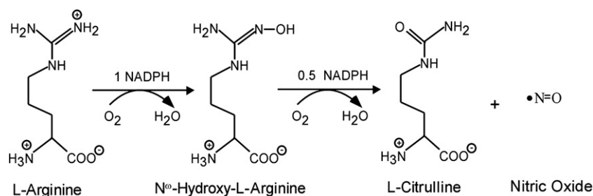
Scheme 1. Biosynthesis of NO from Arginine by NOS enzymes.
