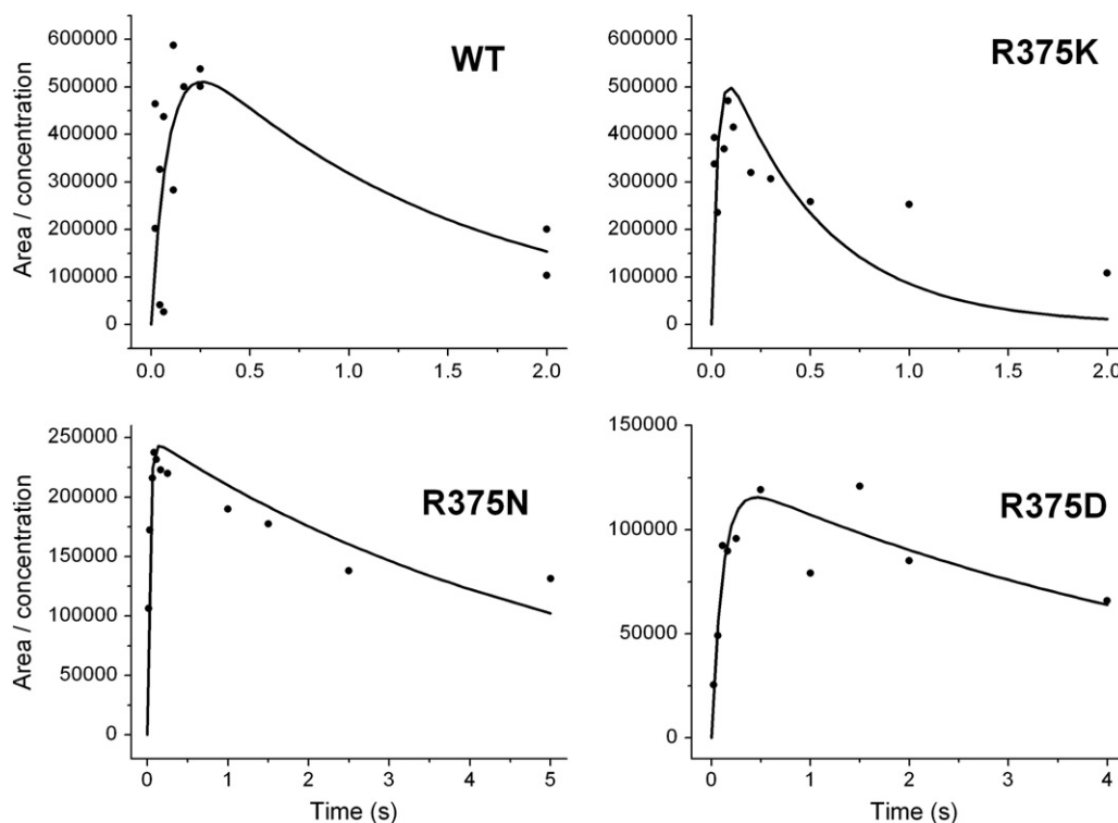
Fig. 10. Calculated concentrations of the H 4 B radical versus time during Arg hydroxylation in Arg375 mutants and wild-type iNOSoxy. The relative concentration of H 4 B radical was calculated by double integration of the EPR signals shown in Fig. 9 and divided by the protein concentration.
