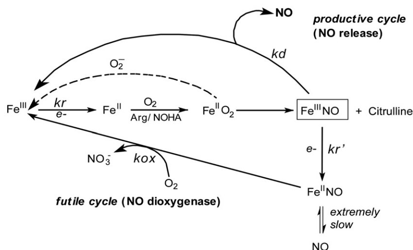
Fig. 6. Global kinetic model for NO synthesis by NOS. During steady state catalysis, the enzyme molecules engage in a productive cycle that releases free NO and in a futile cycle that releases a higher oxide of nitrogen (nitrate). Reduction of ferric enzyme to ferrous ( k_r ) enables the heme to bind O 2 and initiates catalytic reactions. After NO is made, an immediate product of catalysis is the ferric heme-NO complex ( \text{Fe}^{\text{III}}\text{-NO} ), which can either release NO ( k_d ) or become reduced ( k_r' ) to generate a ferrous heme-NO complex ( \text{Fe}^{\text{II}}\text{-NO} ). The ferrous heme-NO complex dissociates extremely slowly and instead regenerates the active ferric enzyme by reacting with O 2 ( k_{ox} ). The \text{Fe}^{\text{II}}\text{O}_2 intermediate can also undergo an uncoupled reaction that generates ferric enzyme and superoxide.
