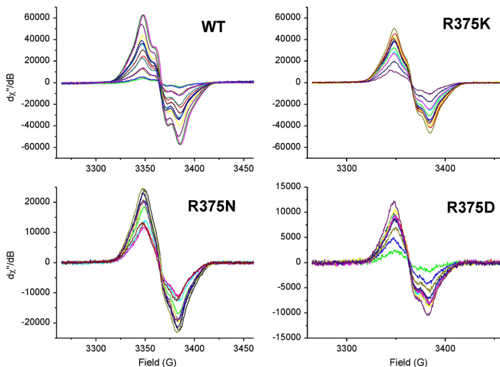
Fig. 9. H 4 B radical formation and decay during Arg hydroxylation in Arg375 mutants and wild-type iNOSoxy. Anaerobic ferrous iNOSoxy proteins were rapidly mixed with an air-saturated solution at 10 °C to start the reaction. Reactions were aged at the various times (16 ms to 5 s), and then quenched by rapid freezing. EPR traces are shown for Arg375 mutants and wild-type iNOSoxy.
