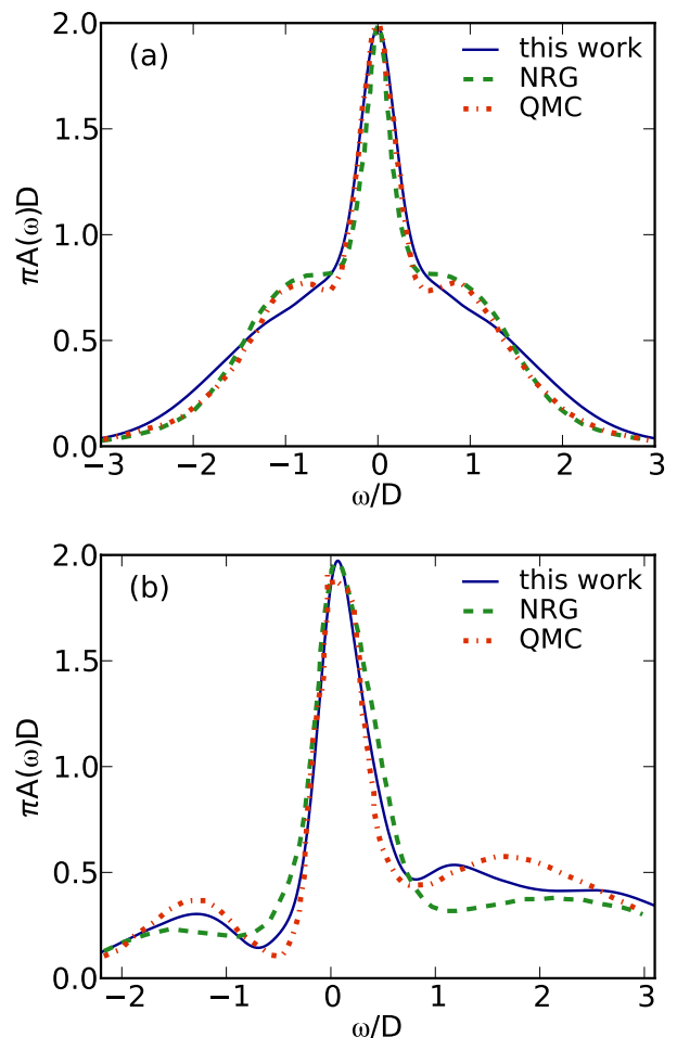
FIG. 8. (Color online) Spectral function for the two-band Hubbard model. Panel (a): U/D = 1.6 , n = 2 (half filling). Panel (b) U/D = 3.8 , n = 1 (quarter filling). In both cases J = \frac{1}{6}U , U' = U - 2J . We fixed a truncation error \varepsilon_{\text{compr}} = 10^{-3} , used a scaling a = 25D , computed N_c = 150 moments and used linear prediction. To represent the two baths, we used two chains of length L = 20 each, obtained with a logarithmic discretization parameter of \Lambda = 2 , leading to grid energies \Lambda^{-n} (see e.g. Ref. 10). The NRG calculation was done for temperature T/D = 0.0025 , the QMC calculation for T/D = 0.01 . Both should be almost indistinguishable from a T = 0 calculation. NRG data from K. Stadler 47 computed with a code of A. Weichselbaum. 48 QMC data from M. Ferrero. 49
