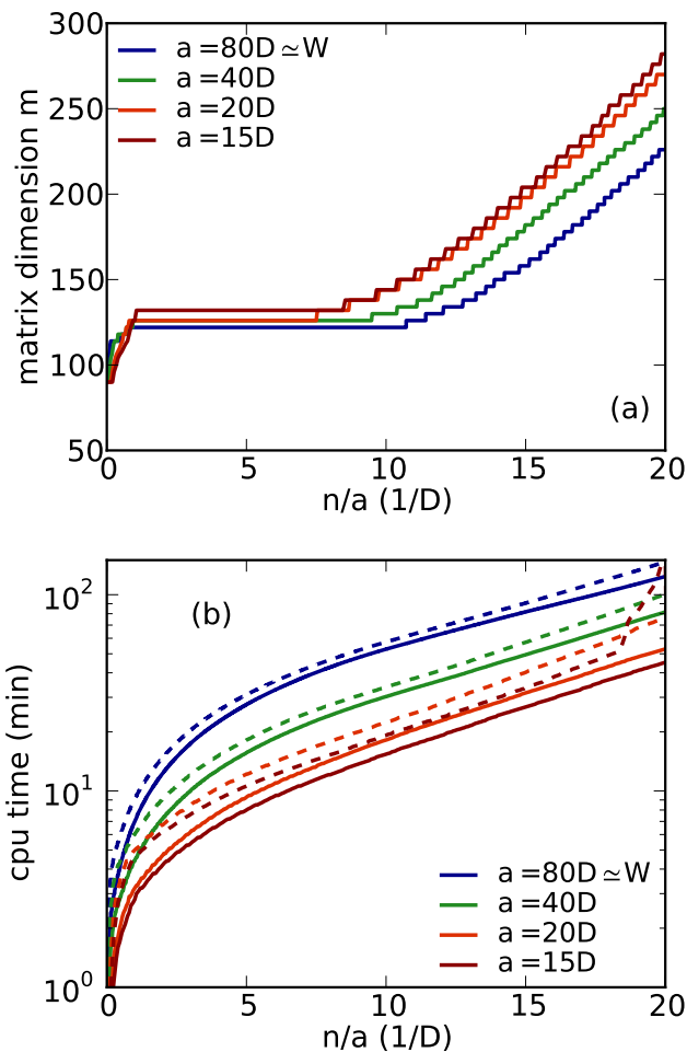
FIG. 3. (Color online) Performance of the adaptive matrix dimension algorithm (Sec. III A) for the example described in the caption of Fig. 2. Panel (a): Adaption of matrix dimensions for different rescaling factors, fixing a truncation error of \epsilon_{\text{compr}} = 10^{-3} . Panel (b): Computer time needed to generate the same amount of information for different scalings running on a single-core 2.0 GHz workstation. Solid lines: fixing a truncation error of \epsilon_{\text{compr}} = 10^{-3} . Dashed lines: \epsilon_{\text{compr}} = 5 \times 10^{-4} . The iteration number where the irregular behavior of the dashed line for a = 15D starts corresponds to the point where numerical errors render the Chebyshev recursion unstable. Note that while small a leads to the largest matrix sizes, which is costly in MPS, the overall cost of CPU time nevertheless is lowest, as a smaller expansion order is needed.
