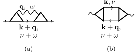
Figure 2. Second-order diagrams contributing to the nonlocal fermionic (a) and bosonic (b) DF self-energy \tilde{\Sigma}_{\mathbf{k}\nu\sigma} and \tilde{\Pi}_{\mathbf{q}\omega} , respectively.
