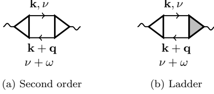
Figure 11. Diagrammatic approximations to the bosonic self-energy \tilde{\Pi}_{\mathbf{q}\omega} .
