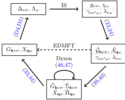
Figure 4. (Color online) Summary of the computational scheme. The loop is started with an initial guess for the hybridization function and retarded interaction. Local observables are calculated in the impurity solver (IS) step. Working with bare dual propagators and neglecting diagrammatic corrections is equivalent to EDMFT (dashed arrow). Corrections beyond EDMFT are taken into account by evaluating diagrams for the dual self-energies, which involve dual propagators and the vertex functions \lambda and \gamma . The diagrams are renormalized self-consistently using Dyson equations. From the dual Green's functions one obtains the physical lattice Green's functions and, in turn, an update for the hybridization and retarded interaction.
