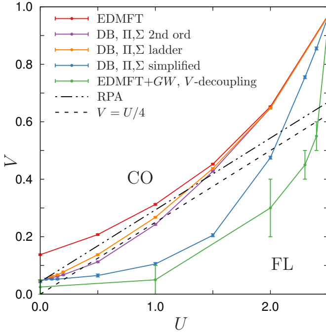
Figure 24. (Color online) U - V phase diagram in the DB approximation with and without vertex corrections and from EDMFT + GW in the V -decoupling scheme. The EDMFT + GW data obtained in the V -decoupling scheme are taken from Ref. 34 (for T = 0.01 ). Approximations that neglect the fermionic frequency structure of the three-leg vertex deviate strongly from those with vertex corrections and from the V = U/4 line, close to where the true phase boundary is expected. For details, see text.
