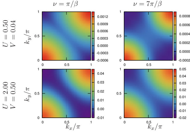
Figure 22. (Color online) Momentum dependence of the non-local part of physical self-energy \text{Im } \Sigma_{\mathbf{k}\nu} - \text{Im } \Sigma_{\nu}^{\text{EDMFT}} for fixed Matsubara frequencies \nu = \pi/\beta (left column) and \nu = 7\pi/\beta (right column) in the ladder approximation. In EDMFT, this quantity is a constant (equal to zero).
