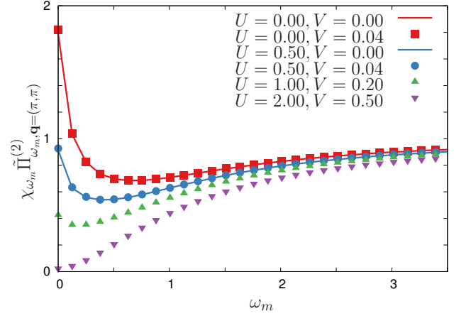
Figure 18. (Color online) The diagrammatic correction \chi_{\omega} \tilde{\Pi}_{\omega, \mathbf{q}=(\pi, \pi)}^{(2)} (see text) in second-order approximation, evaluated at the wave vector associated with charge order and shown as a function of Matsubara frequency. With increasing values of U , the diagrammatic correction is reduced. Its value is only weakly dependent on V .
