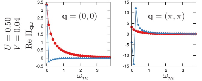
Figure 26. (Color online) Frequency dependence of the physical polarization \Pi_{\mathbf{q}\omega} for fixed momentum \mathbf{q} = (0, 0) (left) and \mathbf{q} = (\pi, \pi) (right) for s-DB (blue, triangles) and EDMFT (red, circles). The colors correspond to those in the phase diagram of Fig. 24. The same quantity in the DB scheme with vertex corrections is shown in Fig. 16.
