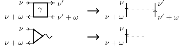
Figure 29. Illustration of how to determine the sign of a diagram. The vertices (left) in a given diagram should symbolically be replaced by interaction lines as indicated on the right. Each closed fermion loop in the resulting diagram contributes a factor -1 . See Appendix B for details.
